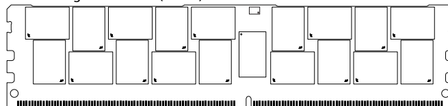
Figure 1: 288-Pin LRDIMM (MO-309, R/C-E1)
