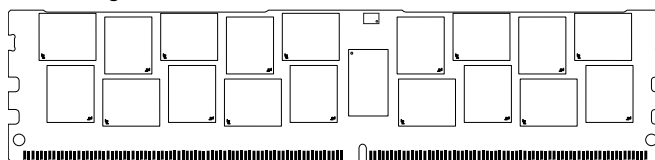
Figure 1: 288-Pin LRDIMM (MO-309, R/C-E)
