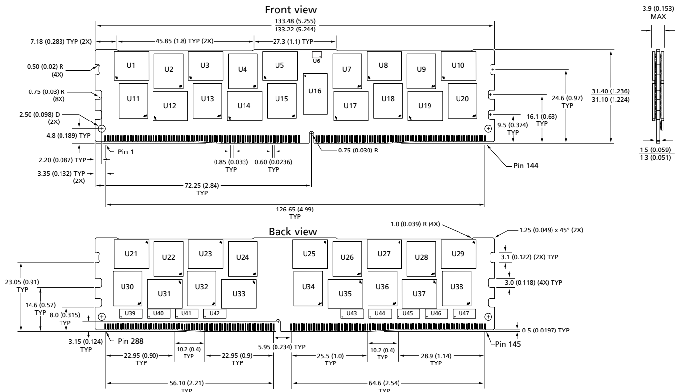
Figure 3: 288-Pin DDR4 LRDIMM
