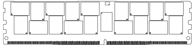
Figure 1: 288-Pin LRDIMM (MO-309, R/C-B)
