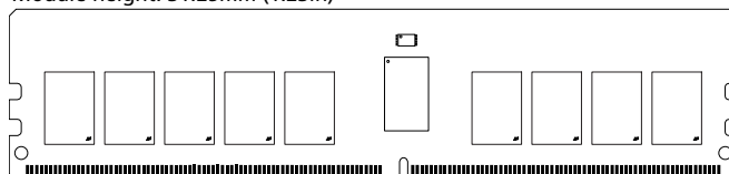
Figure 2: 288-Pin RDIMM (MO-309, R/C-C1)
