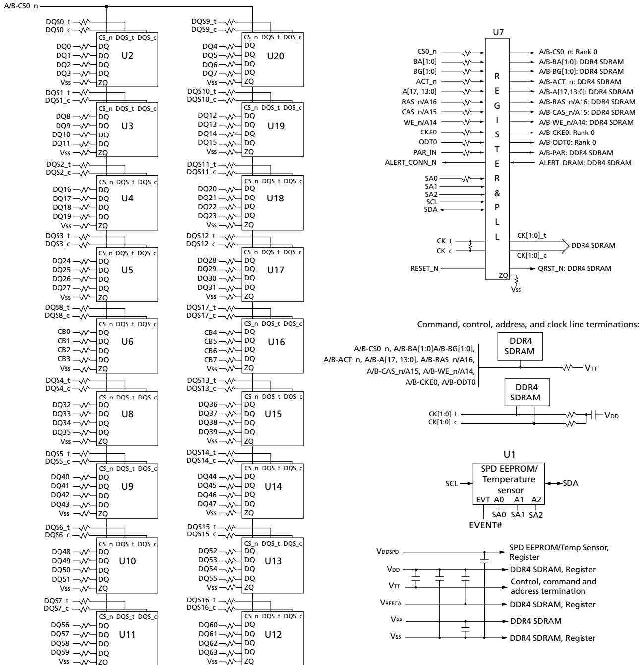
Figure 3: Functional Block Diagram (R/C-C, R/C-C1)
