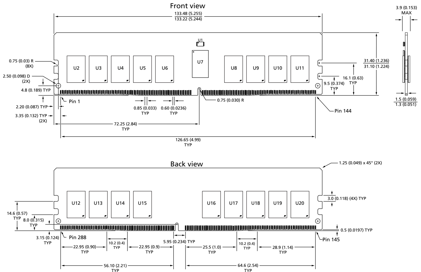
Figure 5: 288-Pin DDR4 RDIMM (R/C-C1)
