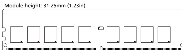
Figure 1: 288-Pin UDIMM (MO-309, R/C-B, R/C-B1)
