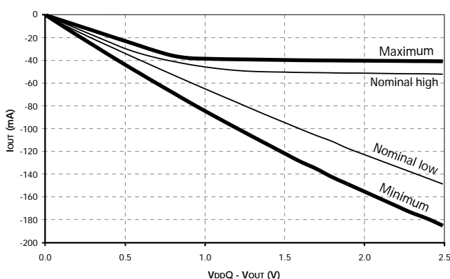
Figure 8: Pull-Up Characteristics
