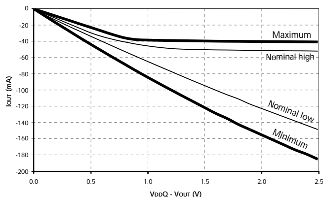
Figure 11: Pull-Up Characteristics
