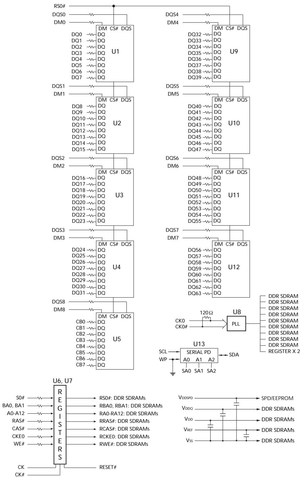
Figure 4: Functional Block Diagram – Low-Profile 512MB
