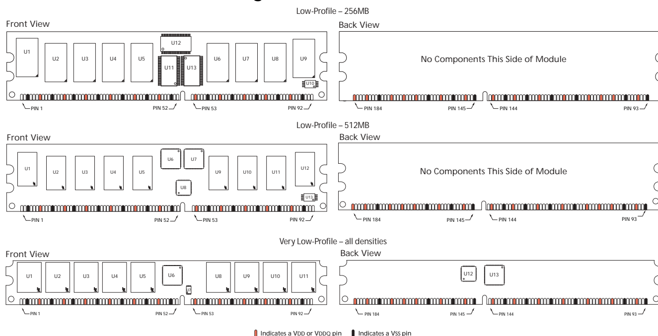
Figure 2: Pin Locations
