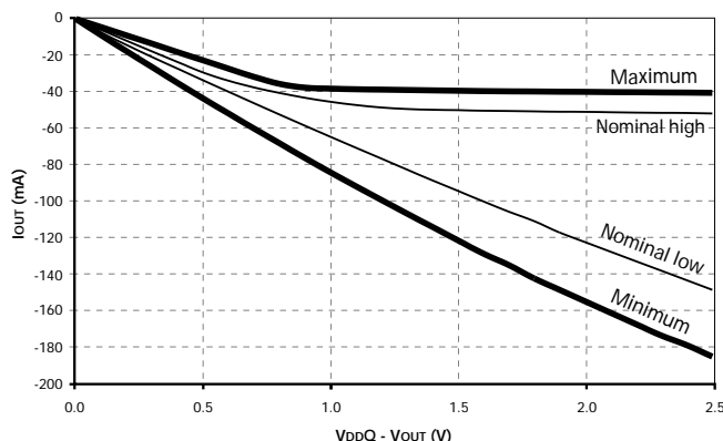
Figure 9: Pull-Up Characteristics
