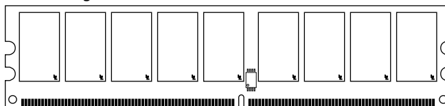
Figure 1: 240-Pin UDIMM (MO-237 R/C A/F)
