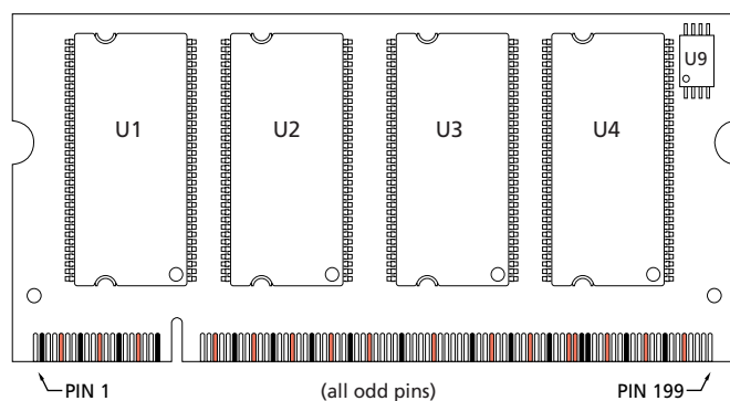
Figure 2: Module Layout
