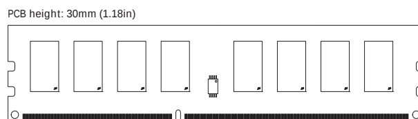
Figure 1: 240-Pin UDIMM (MO-269 R/C A)
