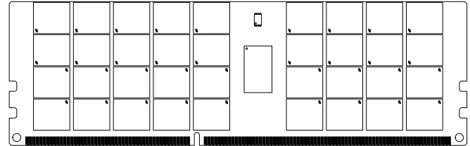
Figure 1: 240-Pin 1.5U RDIMM
