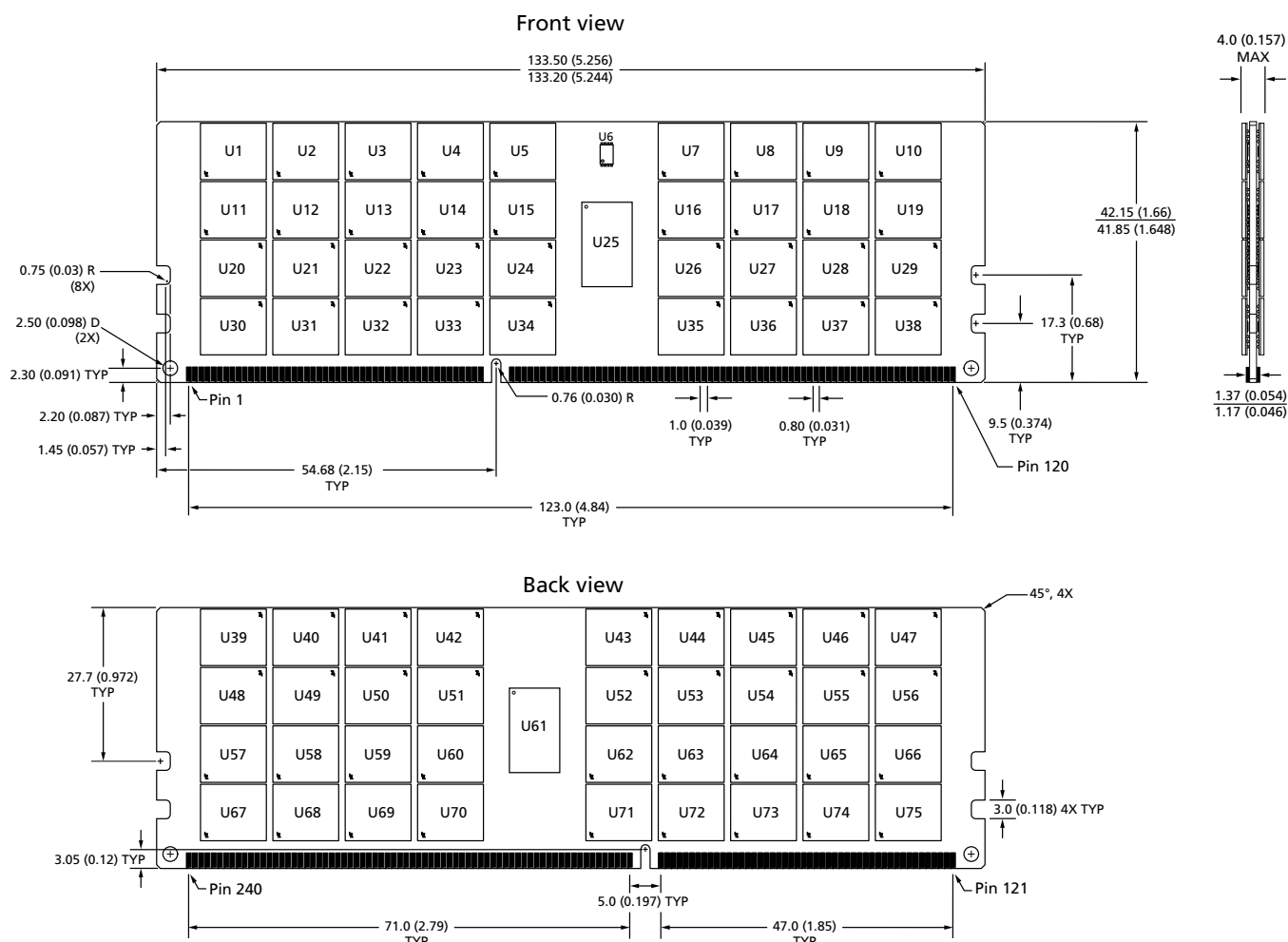
Figure 3: 240-Pin DDR3 RDIMM
