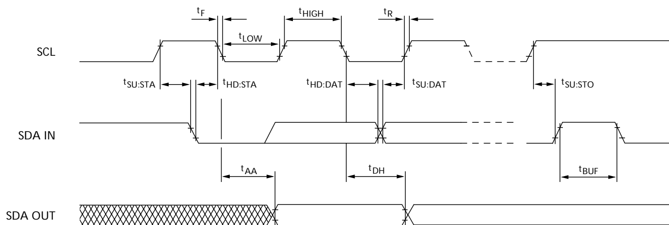
Figure 15: SPD EEPROM Timing Diagram
