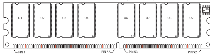
Figure 2: 184-Pin DIMM Pin Locations
