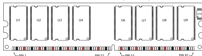
Figure 2: 184-Pin DIMM Pin Locations
