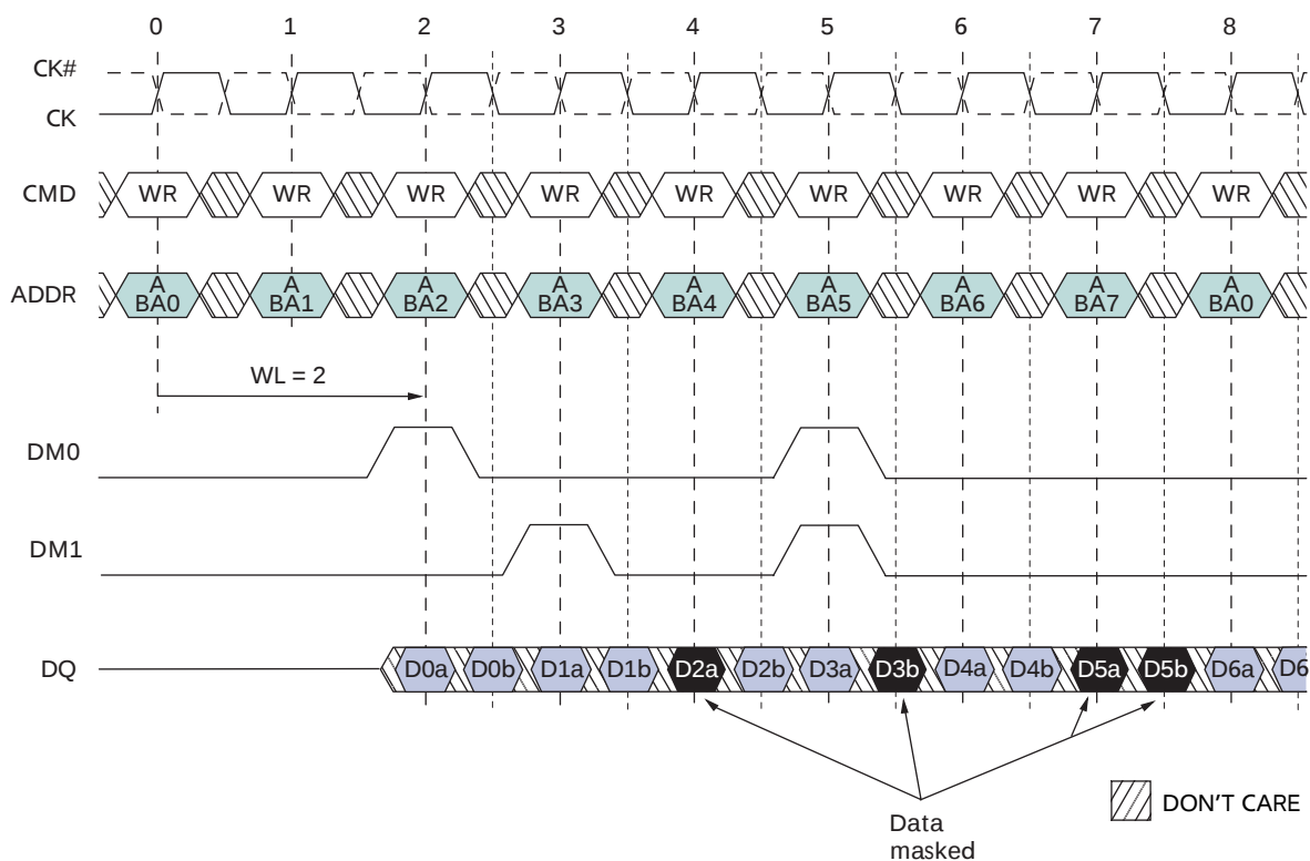
Figure 14: WRITE Data Mask Timing: BL = 2; WL = 2
