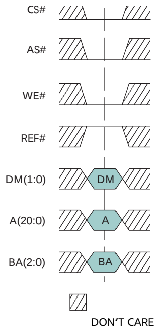
Figure 10: WRITE Command
