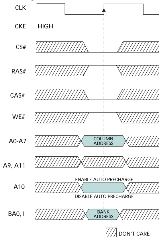
Figure 9: READ Command
