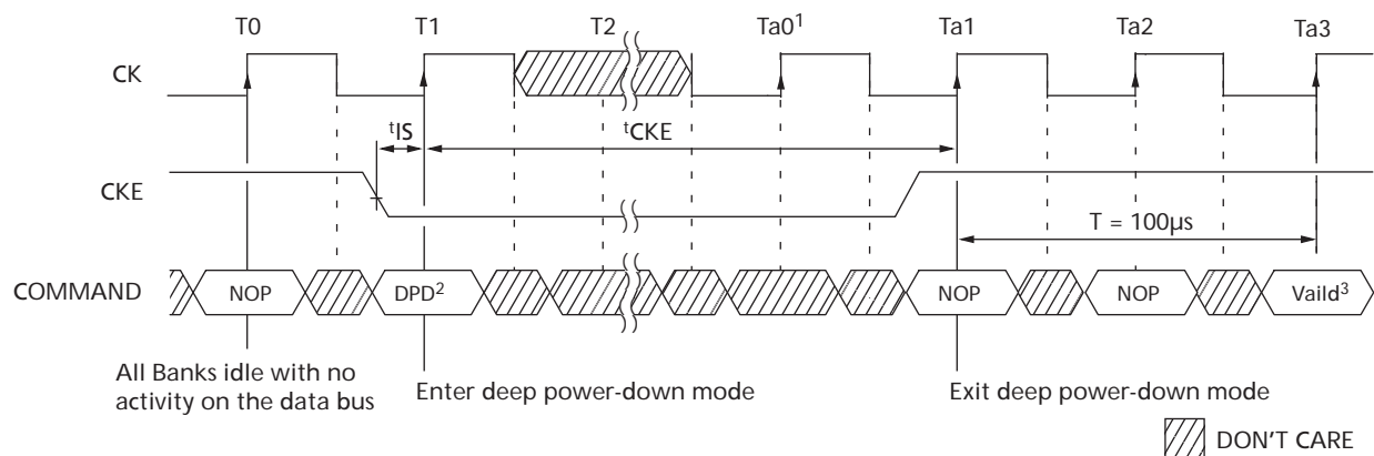
Figure 28: Deep Power-Down
