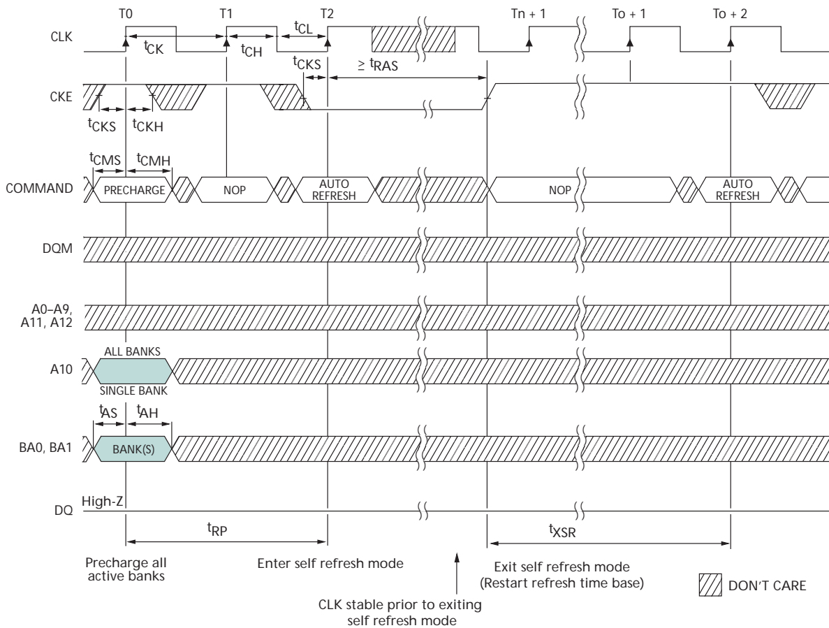
Figure 40: Self Refresh Mode
