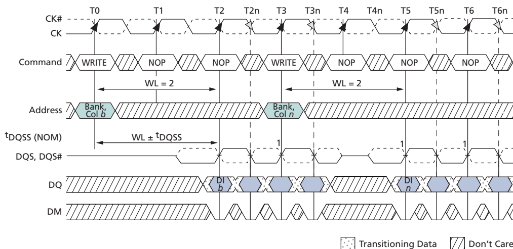
Figure 62: Nonconsecutive WRITE-to-WRITE
