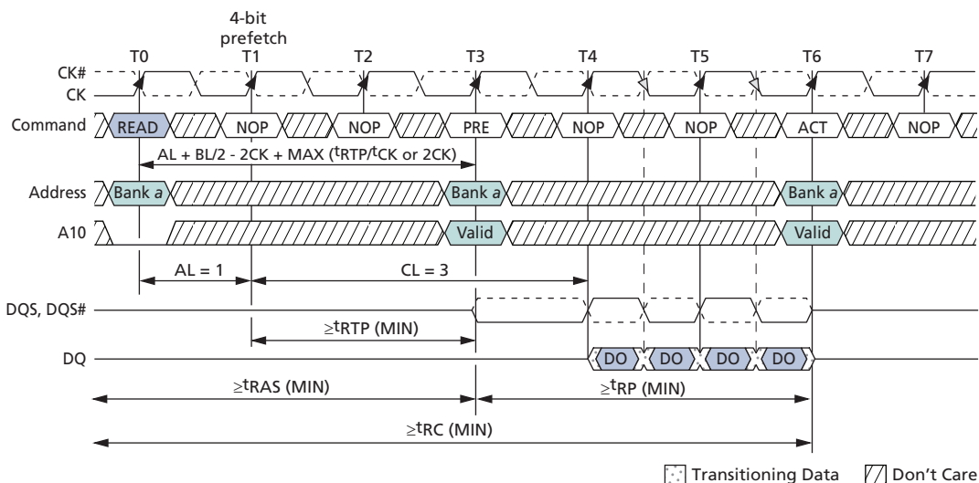
Figure 53: READ-to-PRECHARGE – BL = 4
