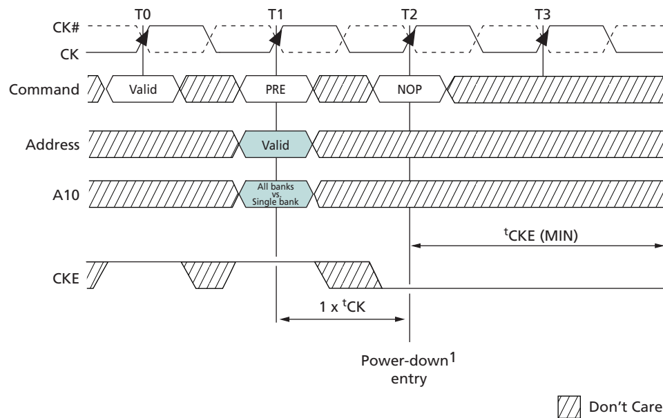
Figure 79: PRECHARGE Command-to-Power-Down Entry
