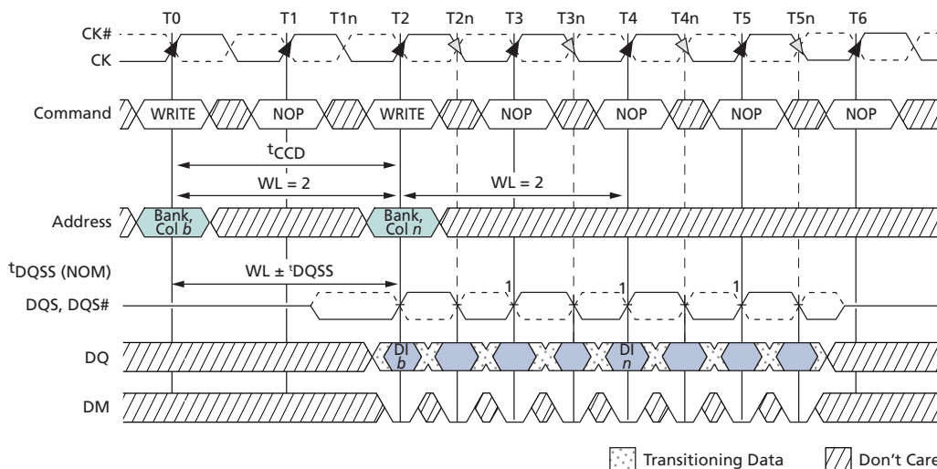
Figure 61: Consecutive WRITE-to-WRITE
