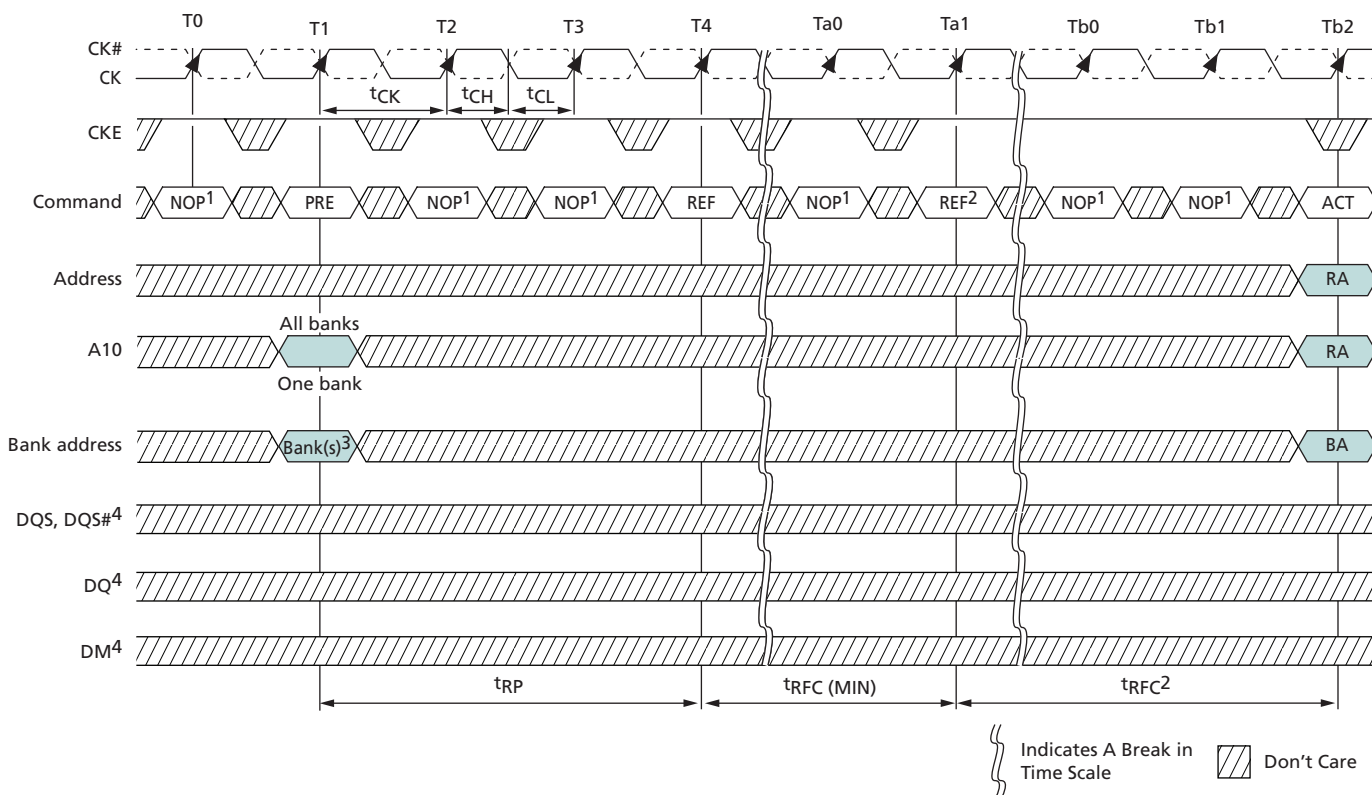
Figure 70: Refresh Mode
