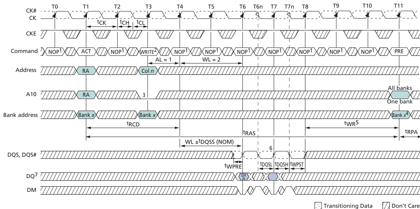
Figure 68: WRITE – DM Operation
