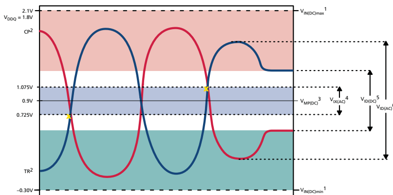
Figure 14: Differential Input Signal Levels
