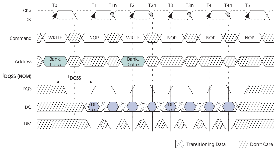
Figure 39: Consecutive WRITE-to-WRITE
