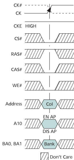
Figure 20: WRITE Command
