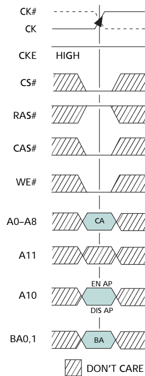
Figure 17: WRITE Command
