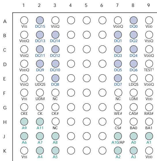
Figure 1: 60-Ball VFBGA Assignment (Top View)
