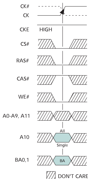
Figure 28: PRECHARGE Command
