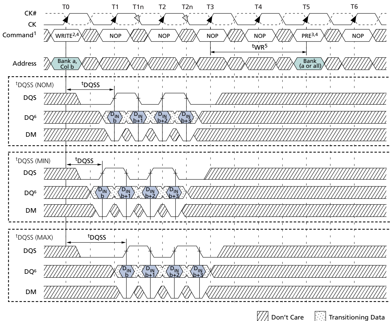
Figure 47: WRITE-to-PRECHARGE – Uninterrupting
