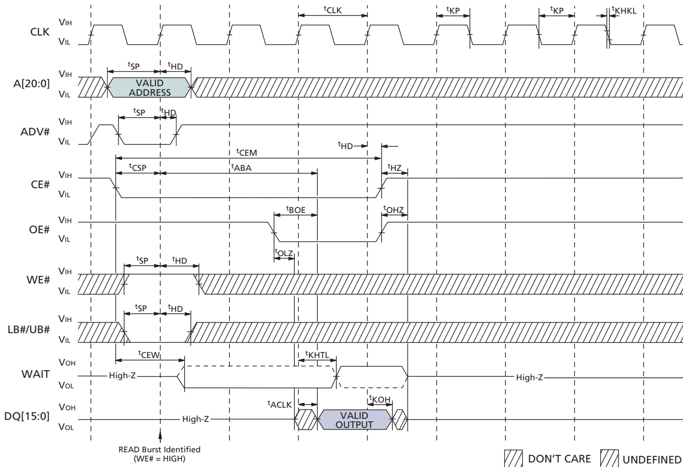
Figure 31: Single-Access Burst READ Operation
