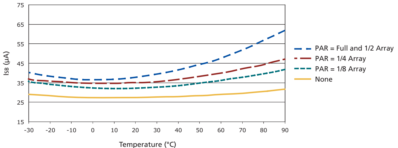
Figure 23: Typical Refresh Current vs. Temperature (Itcr) – 32Mb
