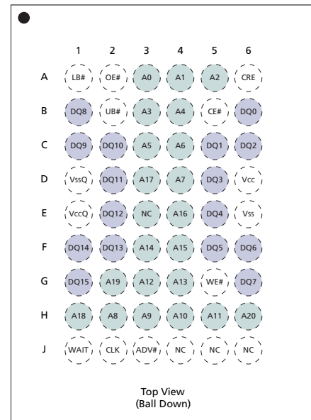
Figure 1: 54-Ball VFBGA
