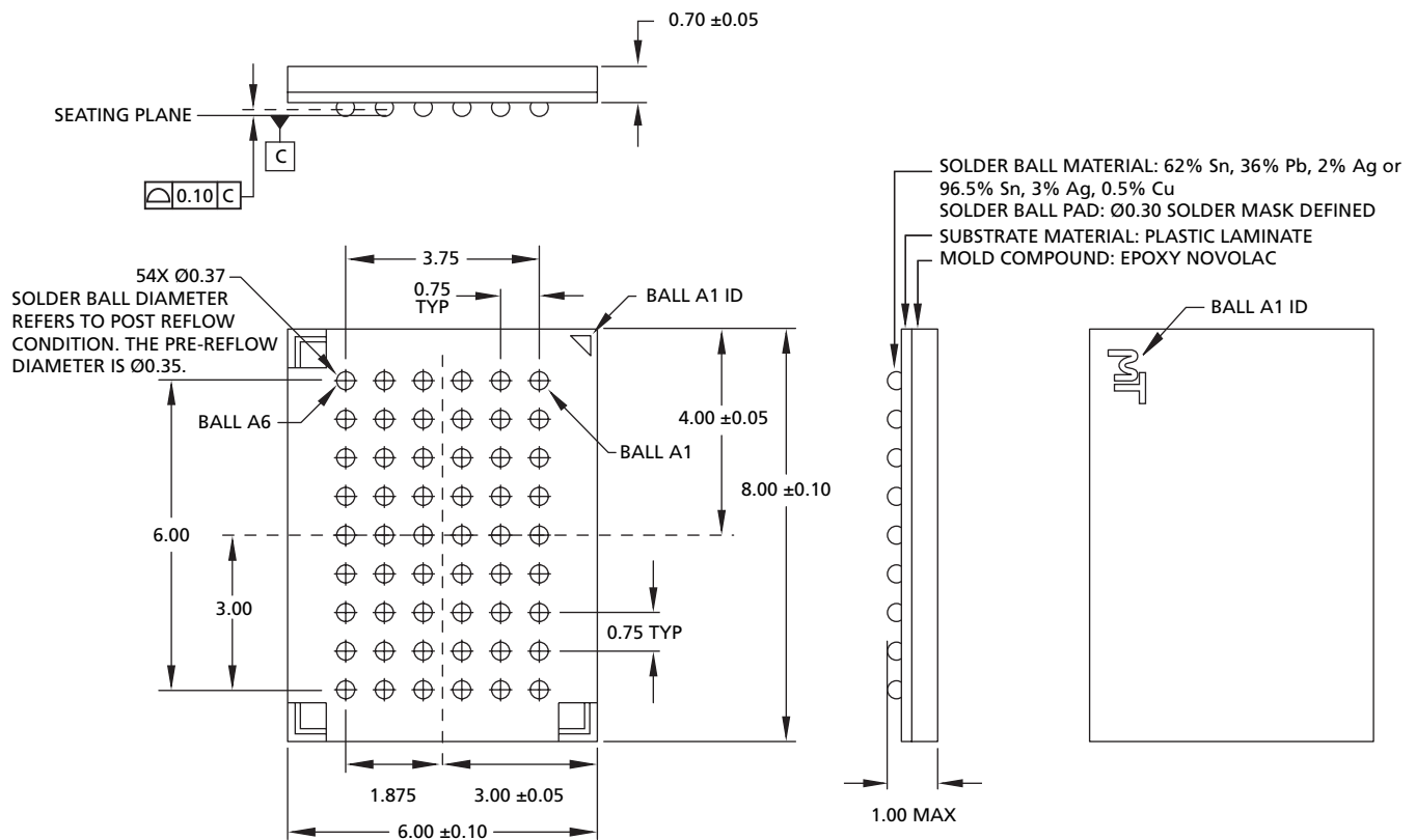
Figure 49: 54-Ball VFBGA
