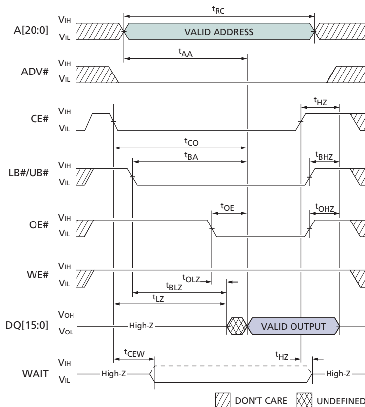
Figure 28: Asynchronous READ
