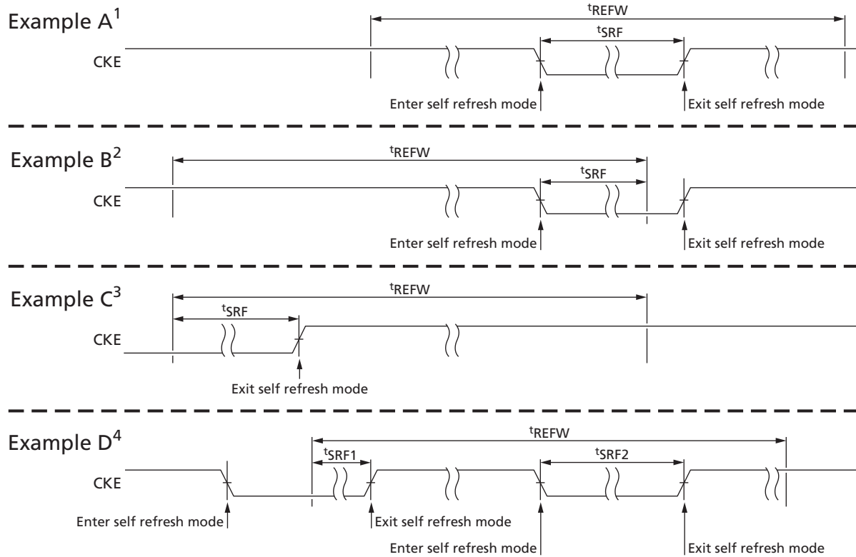
Figure 44: t_{SRF} Definition
