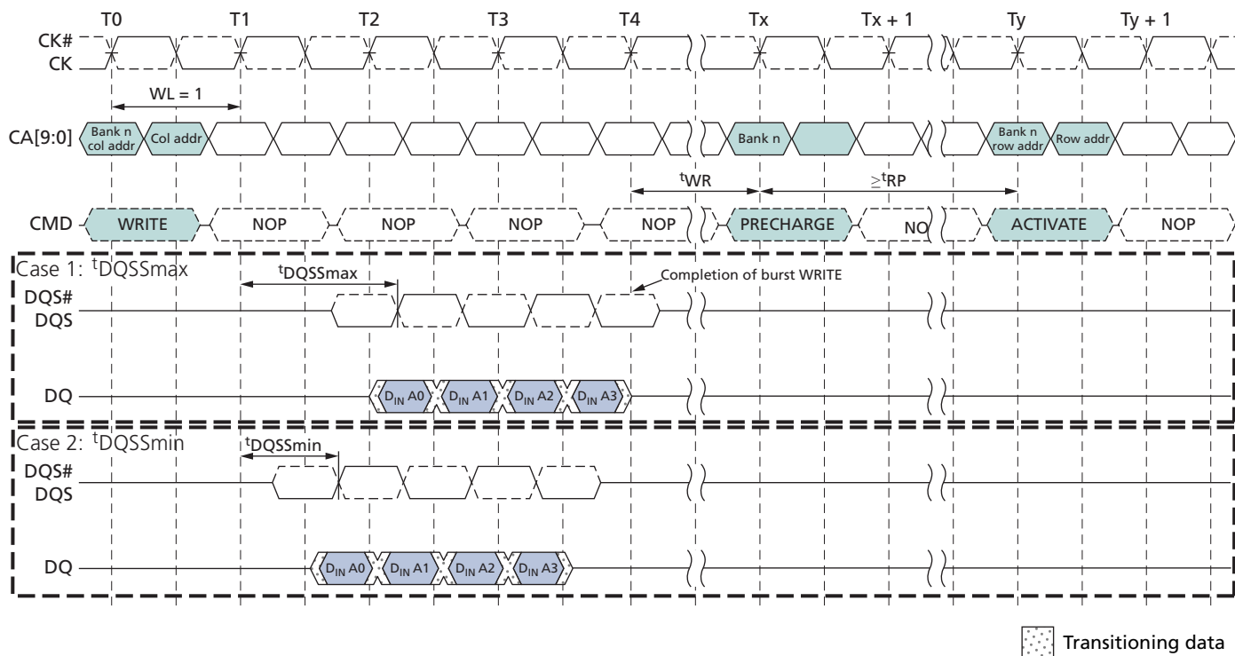
Figure 37: WRITE Burst Followed by PRECHARGE – WL = 1, BL = 4
