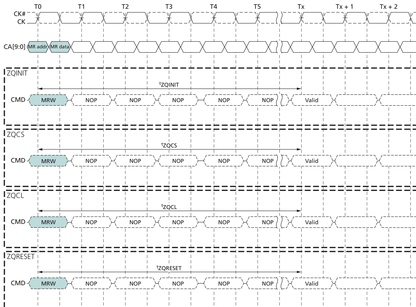
Figure 54: ZQ Timings
