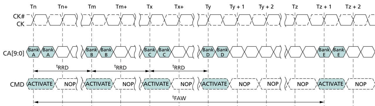
Figure 15: t_{FAW} Timing (8-Bank Devices)
