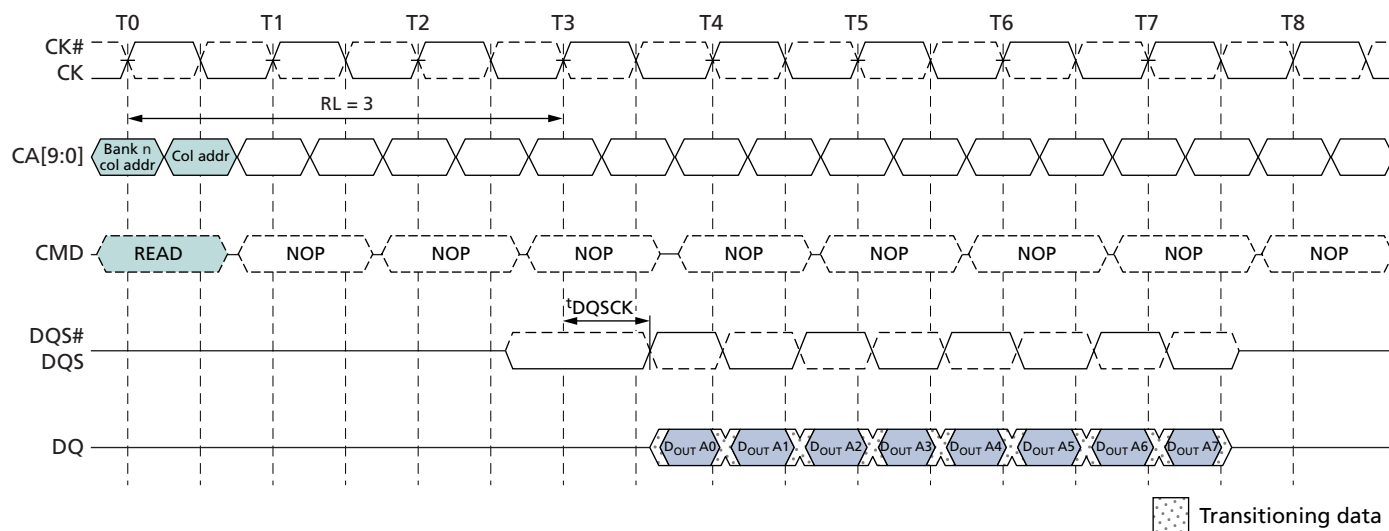
Figure 19: Burst READ – RL = 3, BL = 8, t_{DQSCK} < t_{CK}
