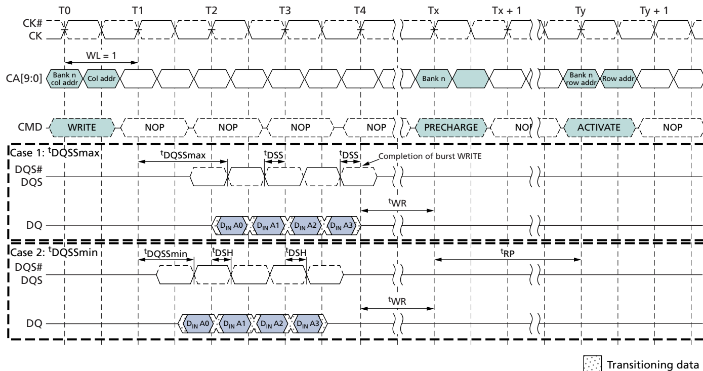
Figure 27: Burst WRITE – WL = 1, BL = 4
