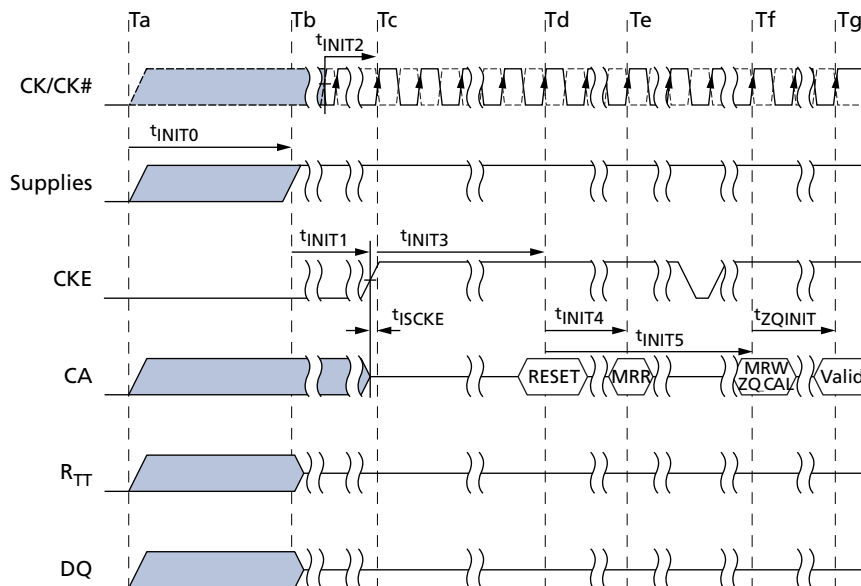
Figure 13: Voltage Ramp and Initialization Sequence
