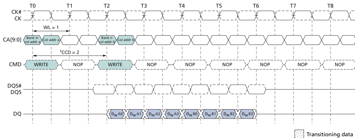
Figure 29: Seamless Burst WRITE – WL = 1, BL = 4, t_{CCD} = 2
