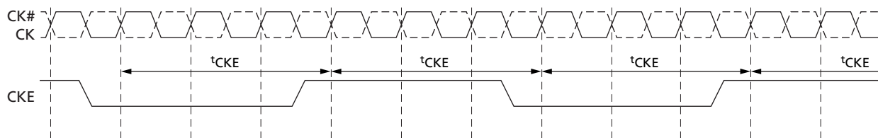
Figure 57: REFRESH-to-REFRESH Timing in CKE Intensive Environments
