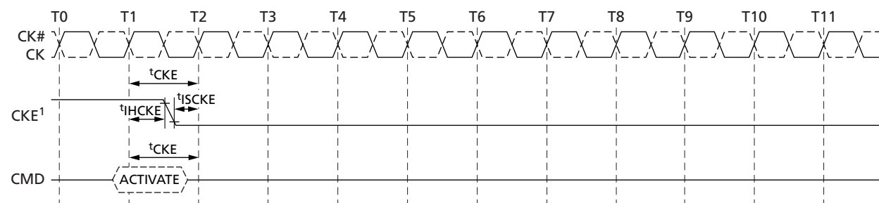
Figure 63: ACTIVATE Command to Power-Down Entry
