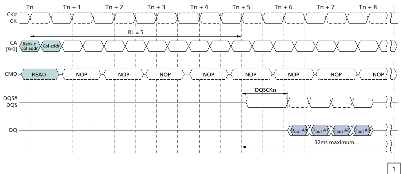
Figure 20: t_{DQSKDL} Timing
