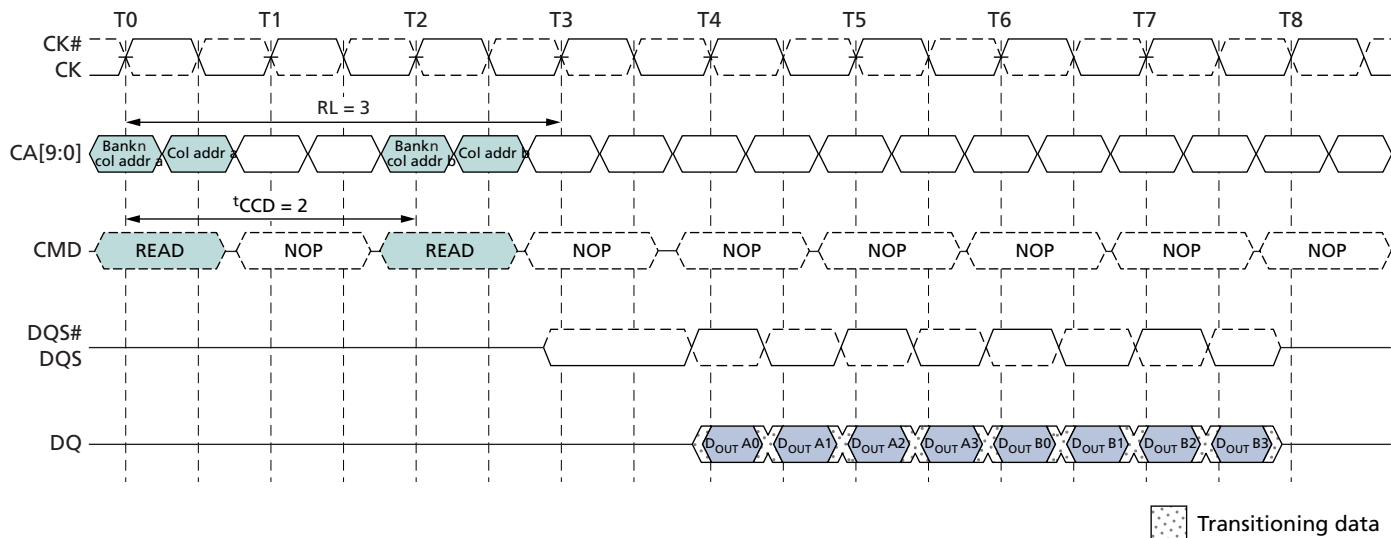
Figure 24: Seamless Burst READ – RL = 3, BL = 4, t_{CCD} = 2
