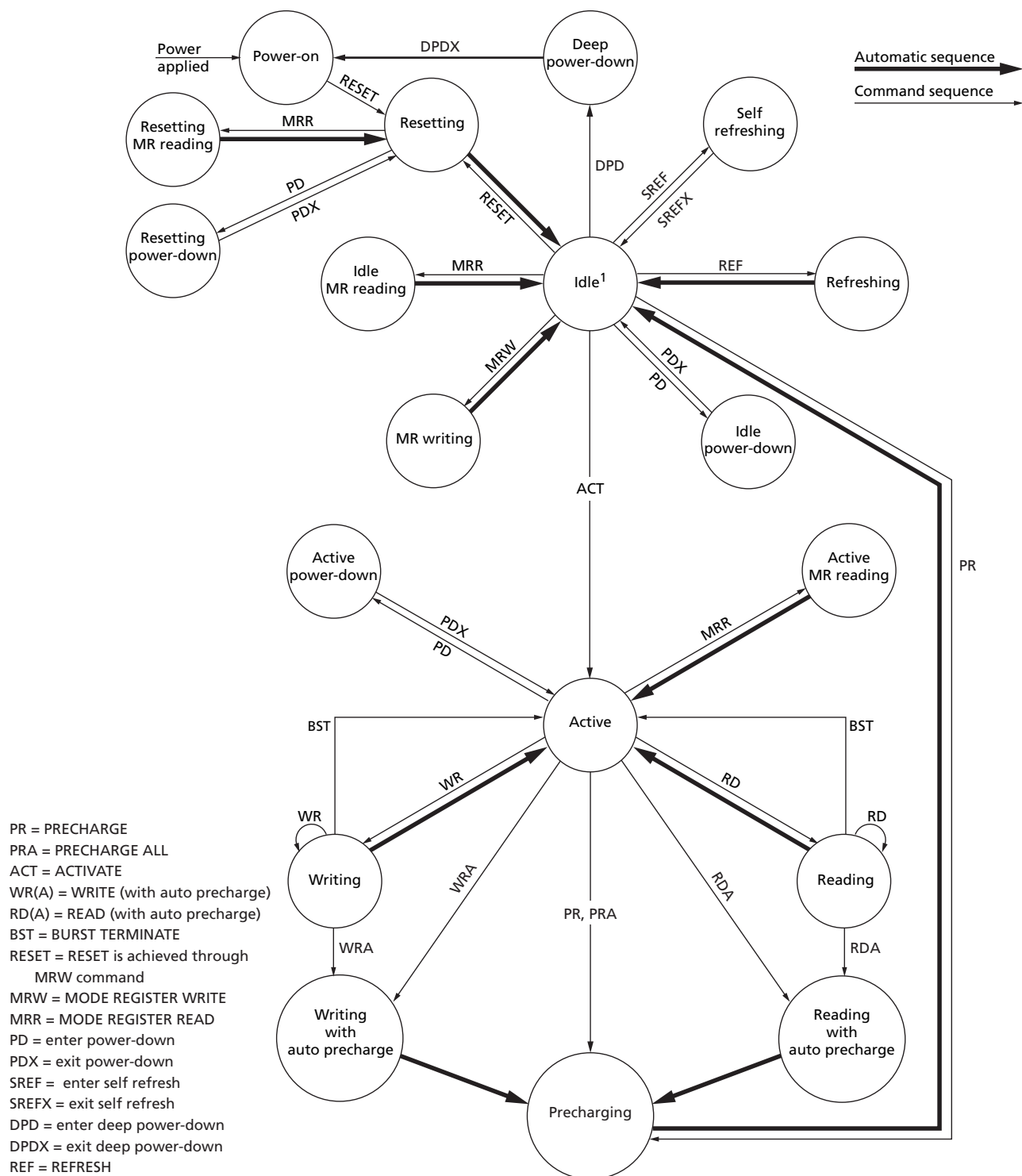
Figure 68: Simplified Bus Interface State Diagram
