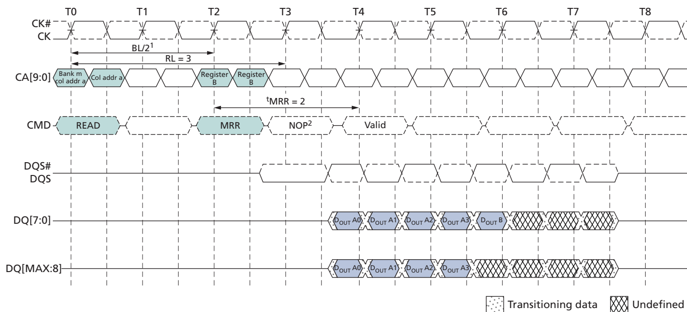
Figure 49: READ to MRR Timing – RL = 3 , t_{MRR} = 2
