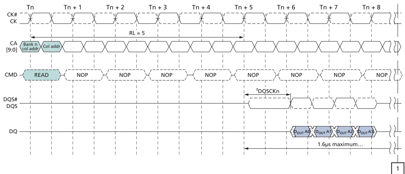
Figure 21: t_{DQSKDM} Timing
