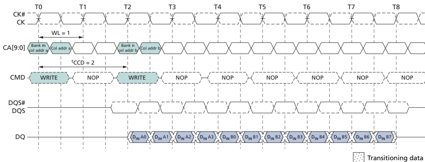
Figure 30: WRITE Burst Interrupt Timing – WL = 1, BL = 8, t_{CCD} = 2
