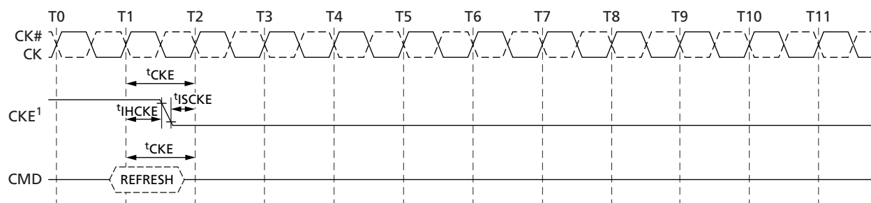
Figure 62: REFRESH Command to Power-Down Entry
