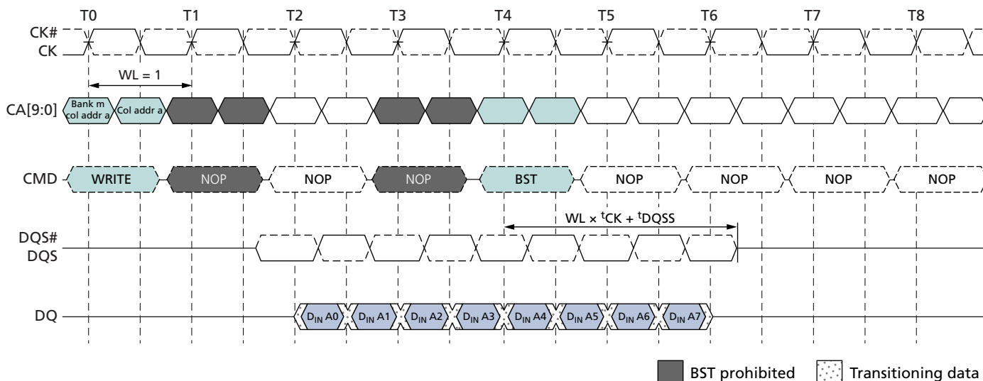
Figure 31: Burst WRITE Truncated by BST – WL = 1, BL = 16
