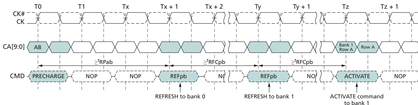
Figure 46: Per-Bank REFRESH Operation
