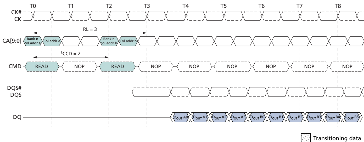
Figure 25: READ Burst Interrupt Example – RL = 3, BL = 8, t_{CCD} = 2
