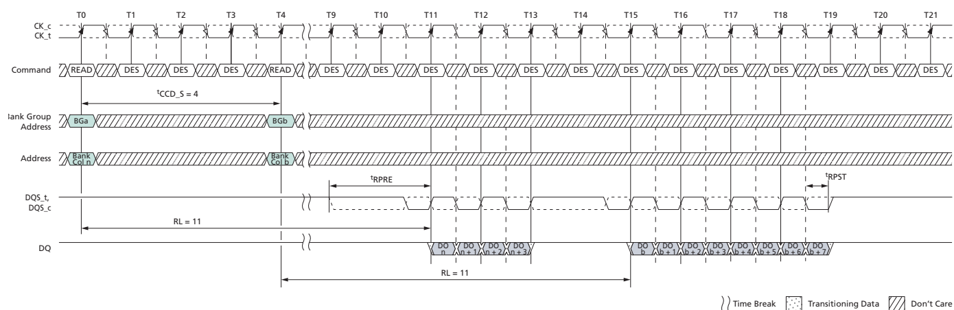
Figure 140: READ (BC4) to READ (BL8) OTF with 2 t CK Preamble in Different Bank Group
