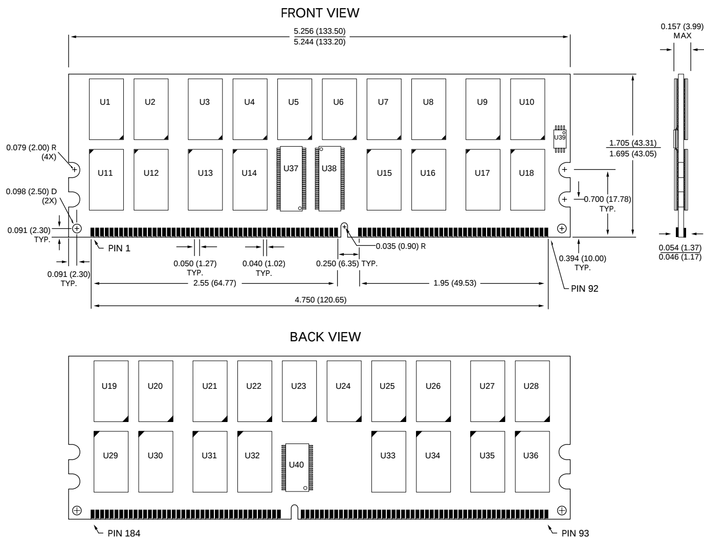
Figure 19: Standard 184-Pin DDR DIMM Dimensions
