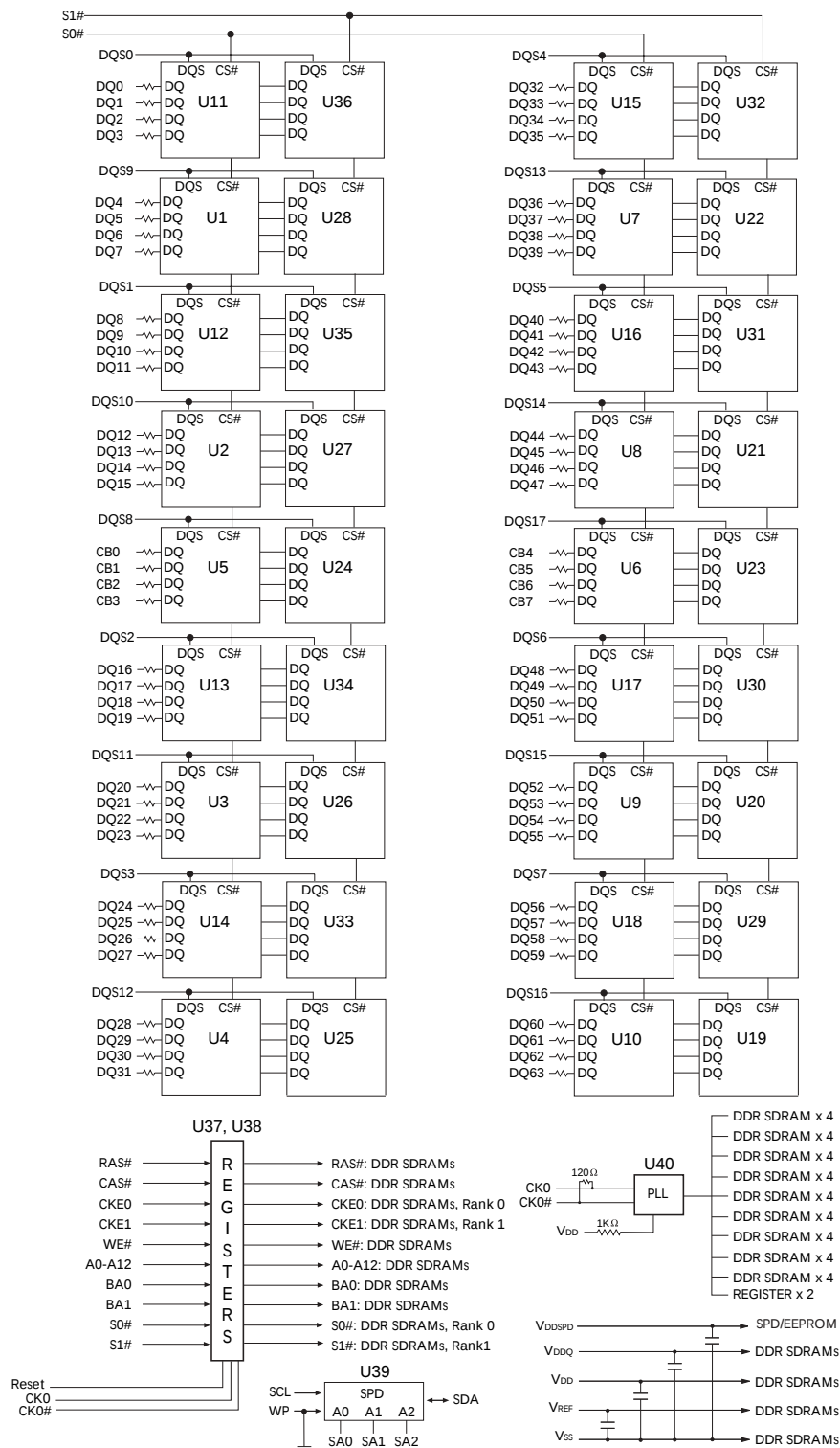
Figure 4: Standard PCB Functional Block Diagram – 1GB, 2GB
