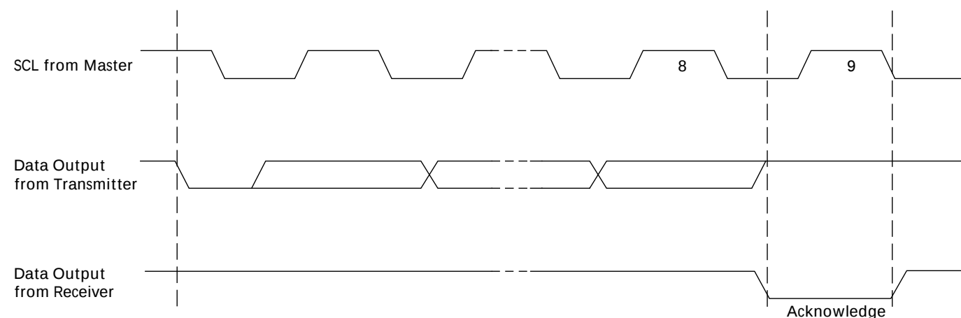
Figure 17: Acknowledge Response From Receiver
