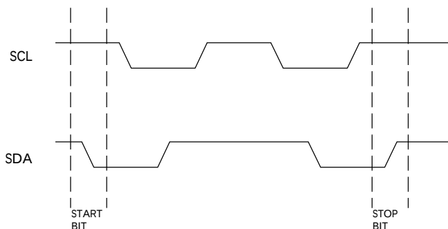
Figure 16: Definition of Start and Stop
