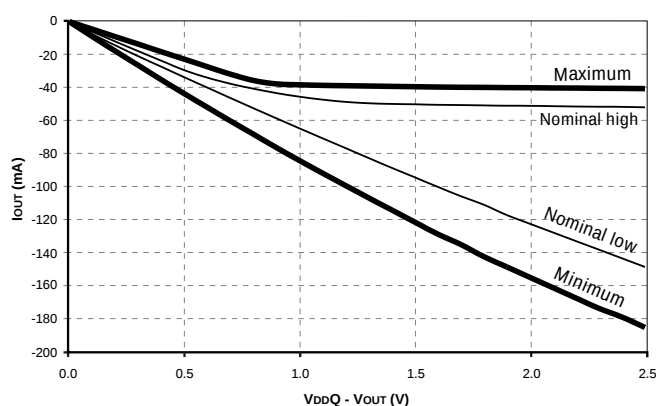
Figure 12: Pull-Up Characteristics
