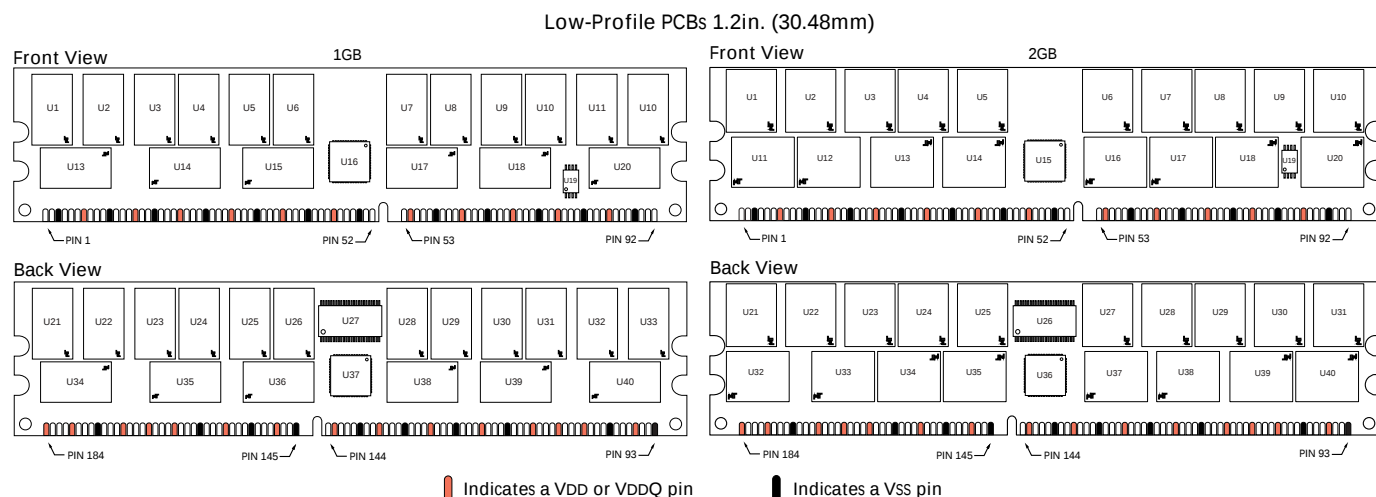
Figure 3: Pin Locations (Low-Profile PCB)
