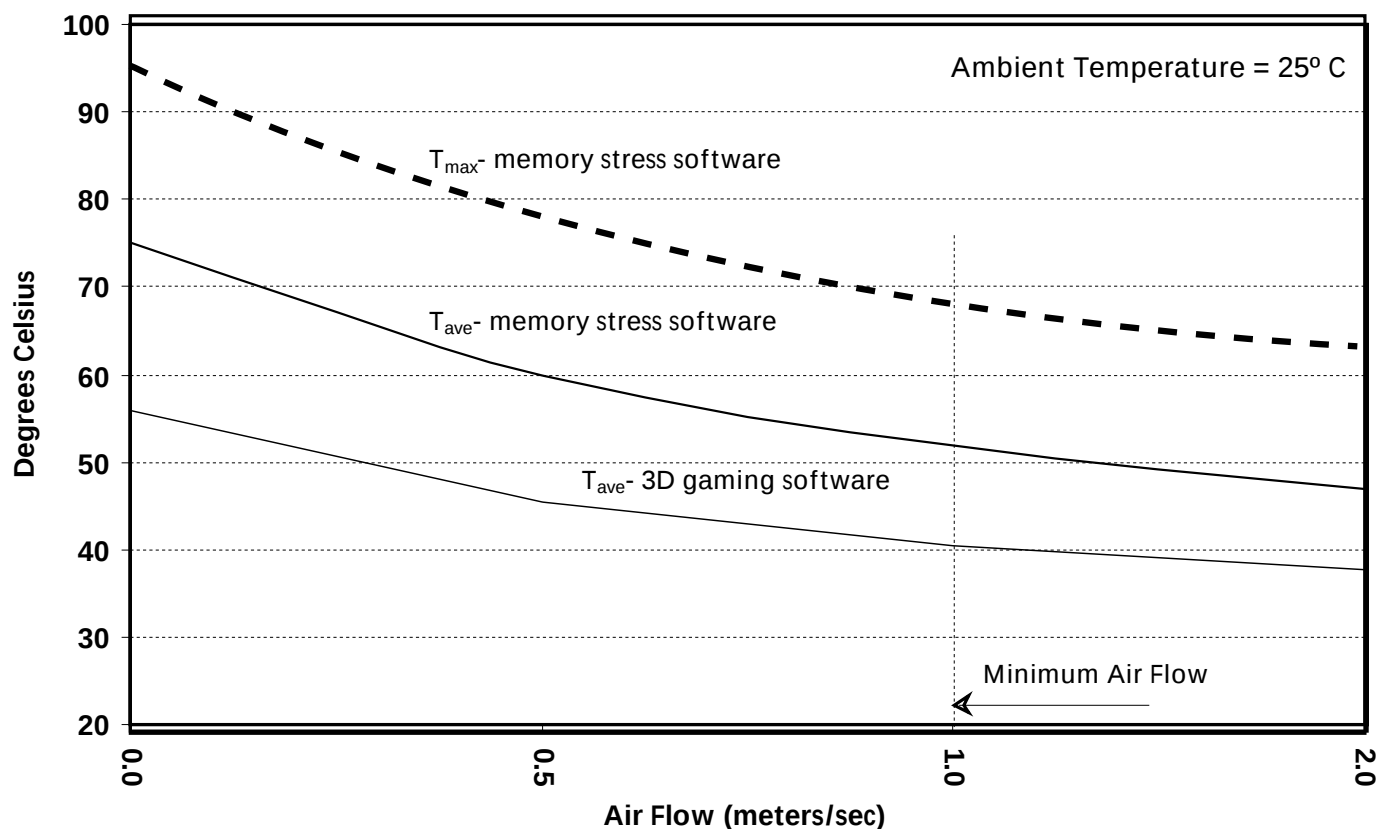
Figure 14: Component Case Temperature vs. Air Flow
