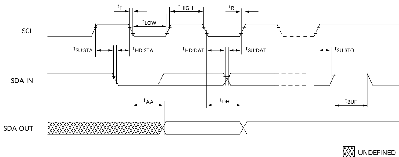
Figure 18: SPD EEPROM Timing Diagram
