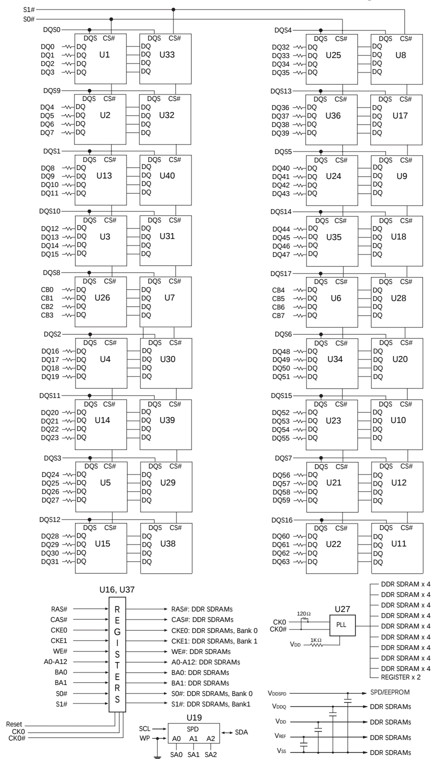
Figure 5: Low-Profile PCB Functional Block Diagram – 1GB
