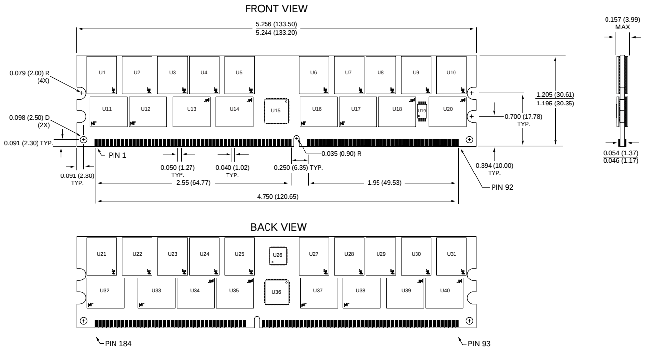
Figure 21: Low-Profile (2GB) 184-Pin DDR DIMM Dimensions
