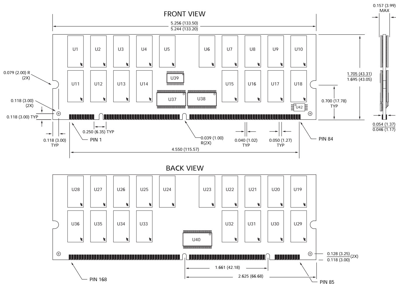
Figure 11: 168-Pin DIMM Dimensions
