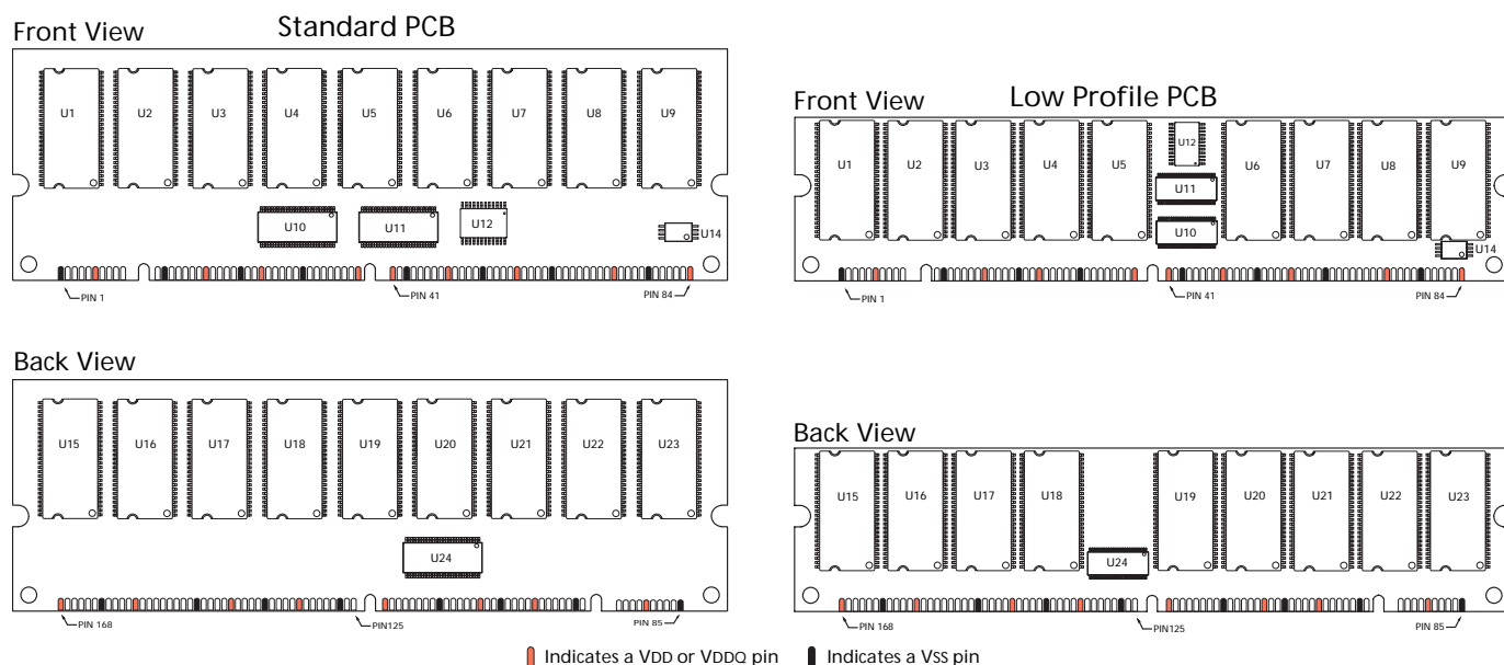
Figure 2: 168-Pin DIMM Pin Locations
