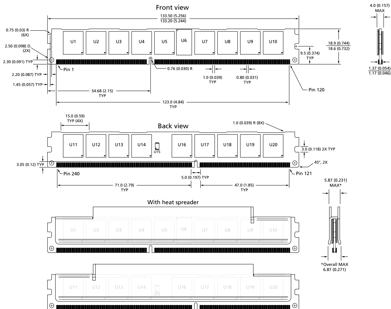
Figure 3: 240-Pin DDR3 RDIMM
