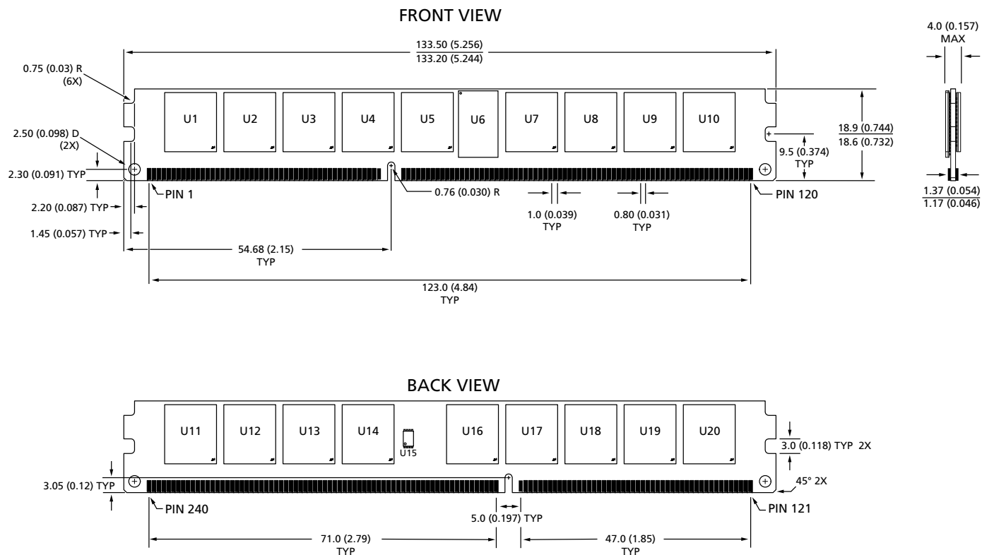
Figure 3: 240-Pin DDR3 RDIMM
