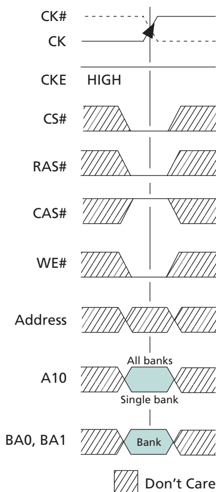
Figure 108: PRECHARGE Command
