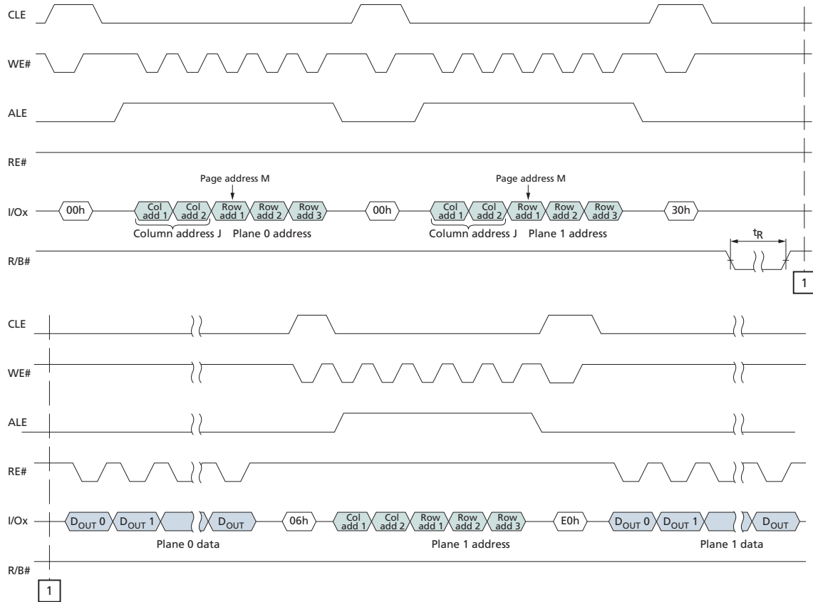
Figure 44: READ PAGE TWO-PLANE (00h-00h-30h) Operation
