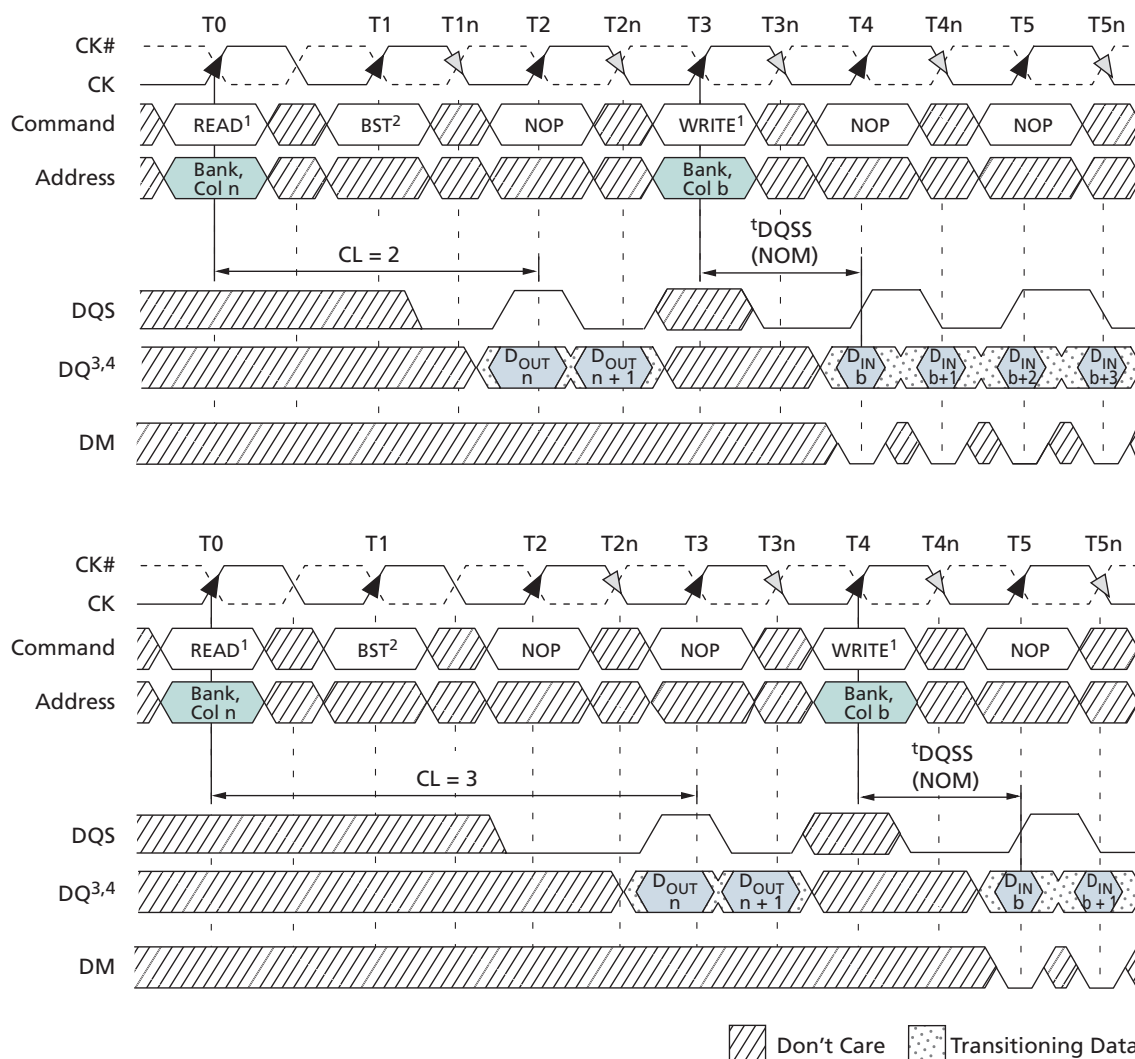
Figure 123: READ-to-WRITE
