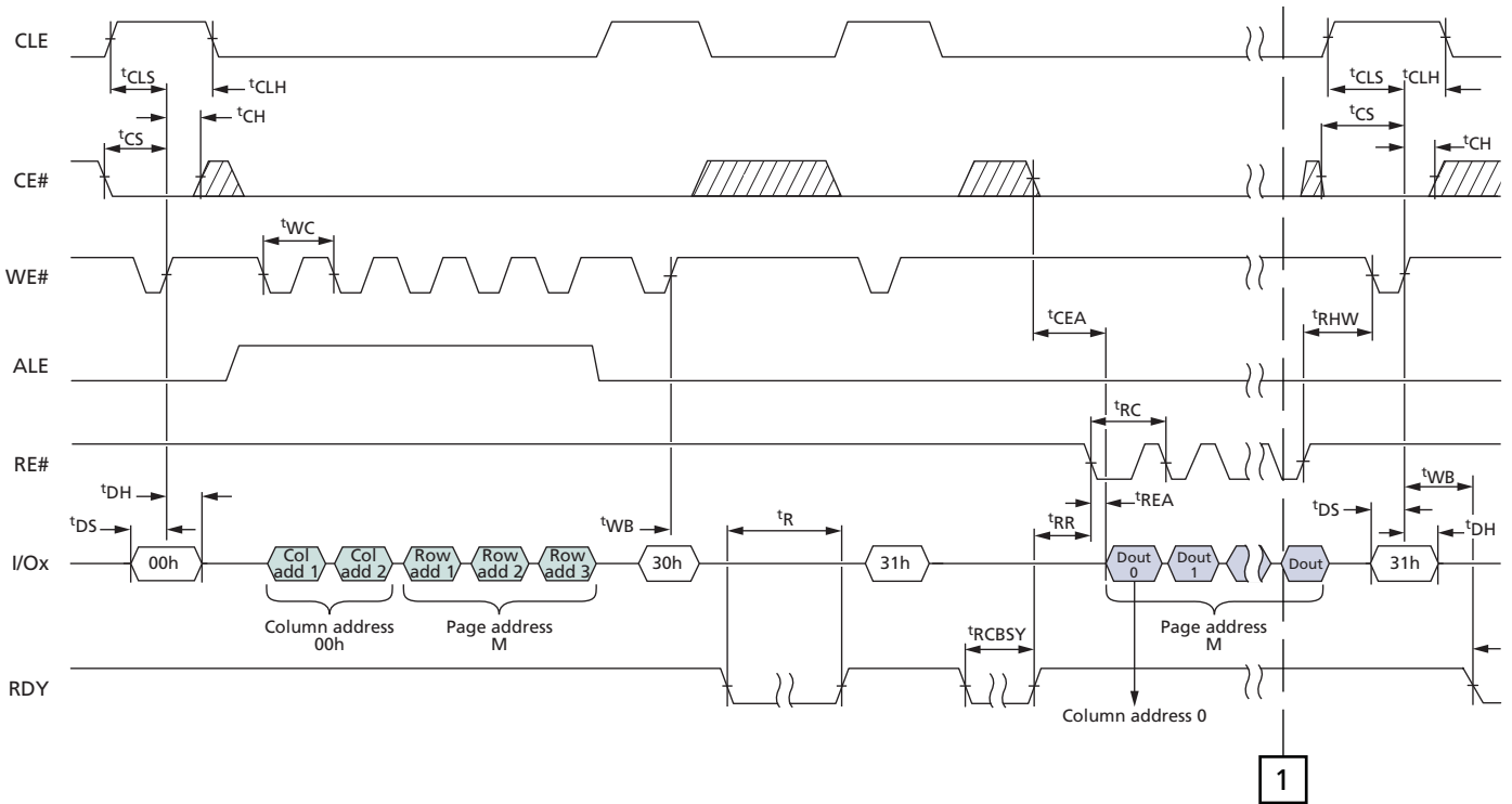
Figure 90: READ PAGE CACHE SEQUENTIAL
