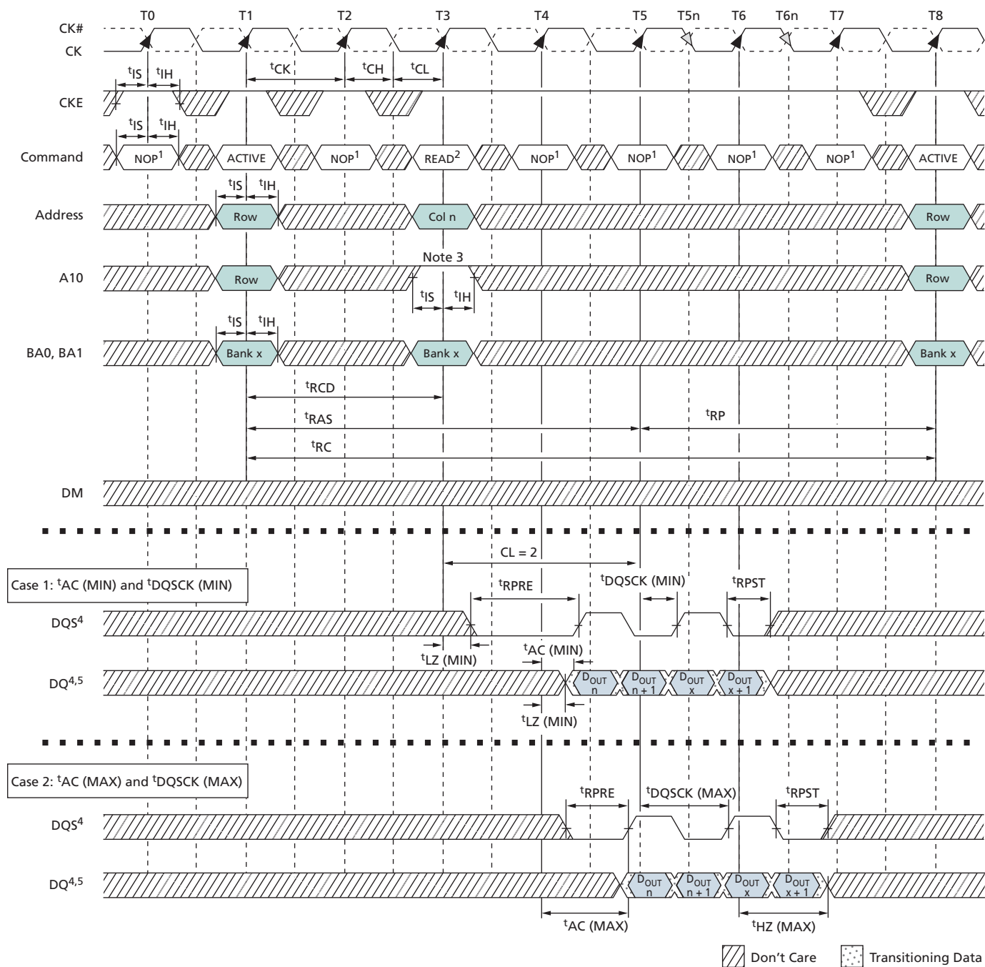
Figure 140: Bank Read – With Auto Precharge
