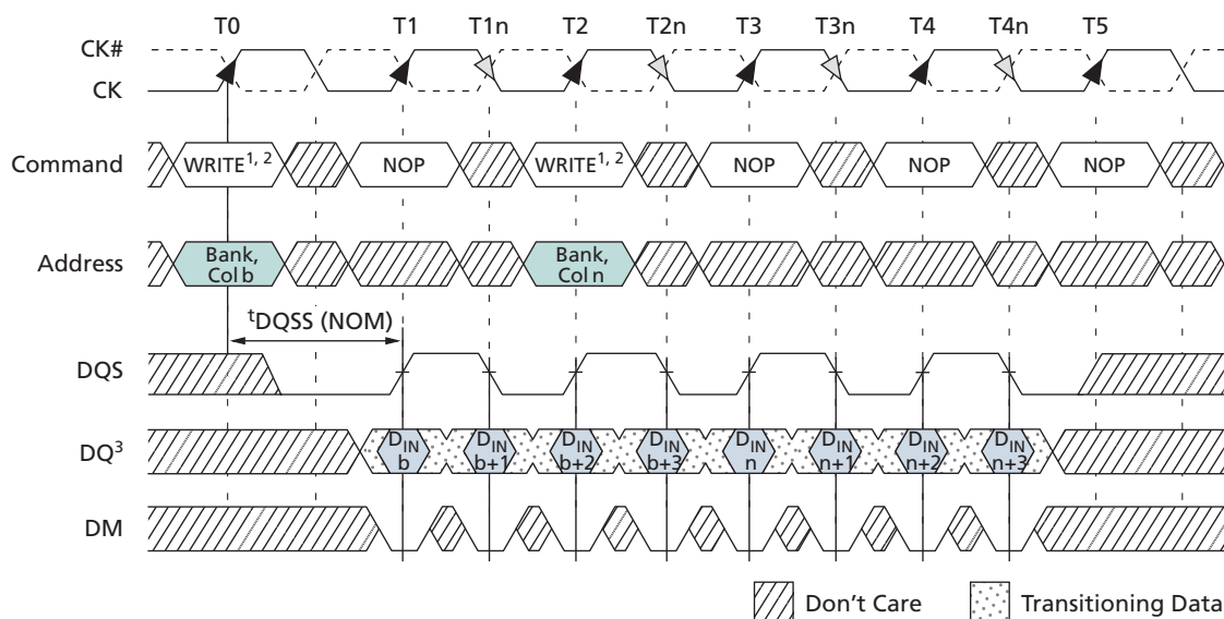
Figure 131: Consecutive WRITE-to-WRITE
