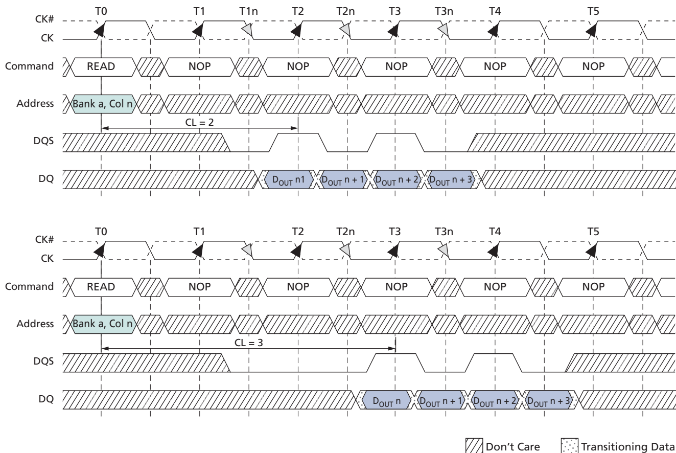
Figure 118: READ Burst
