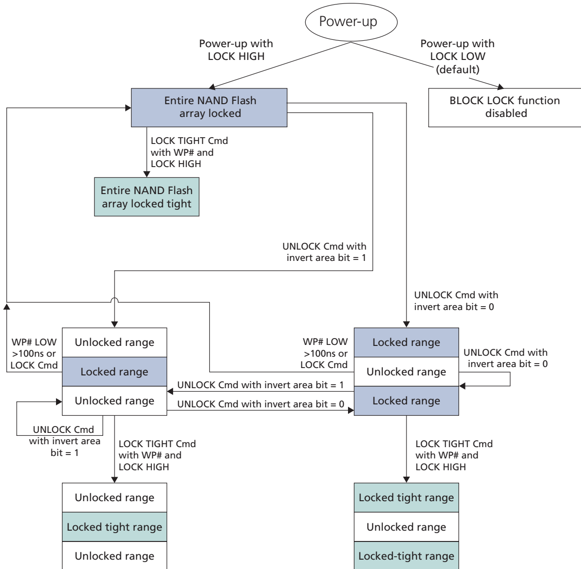
Figure 65: BLOCK LOCK Flowchart
