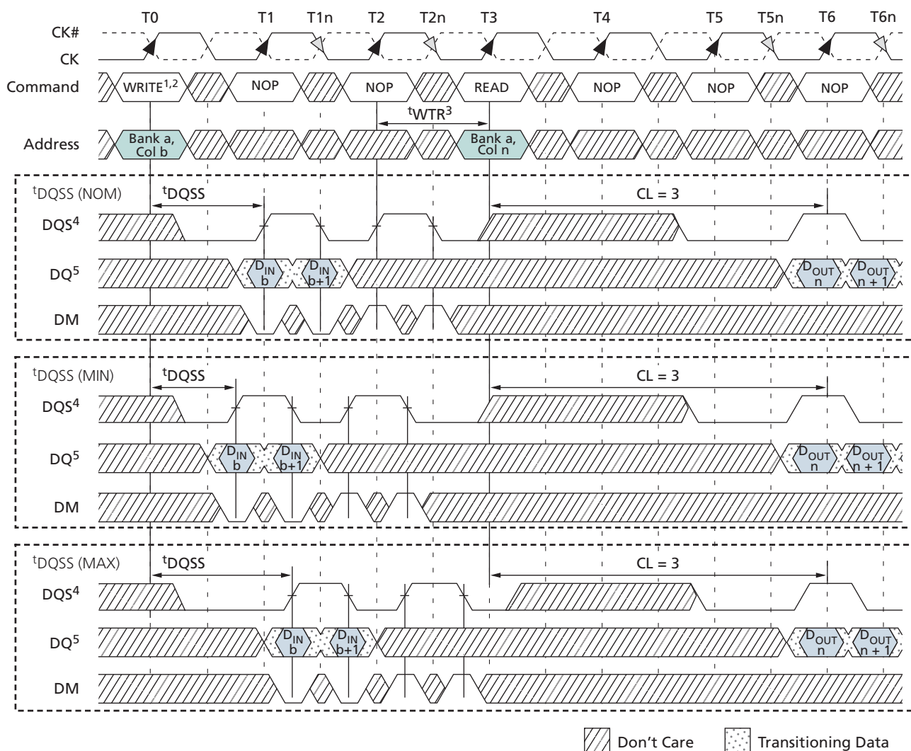
Figure 135: WRITE-to-READ – Interrupting
