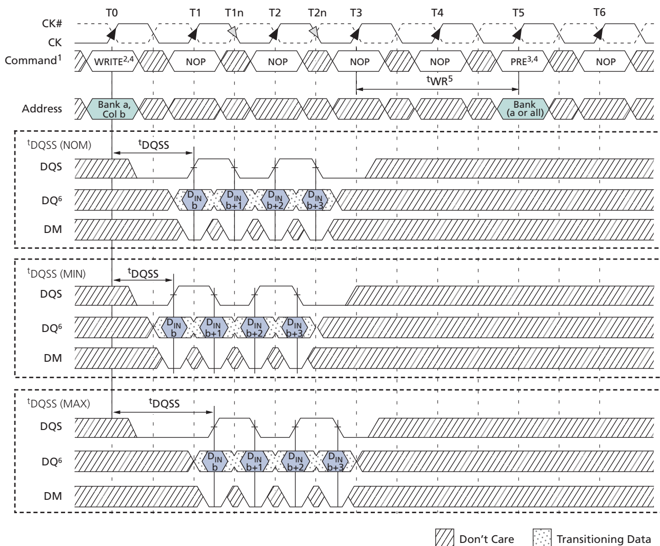
Figure 137: WRITE-to-PRECHARGE – Uninterrupting
