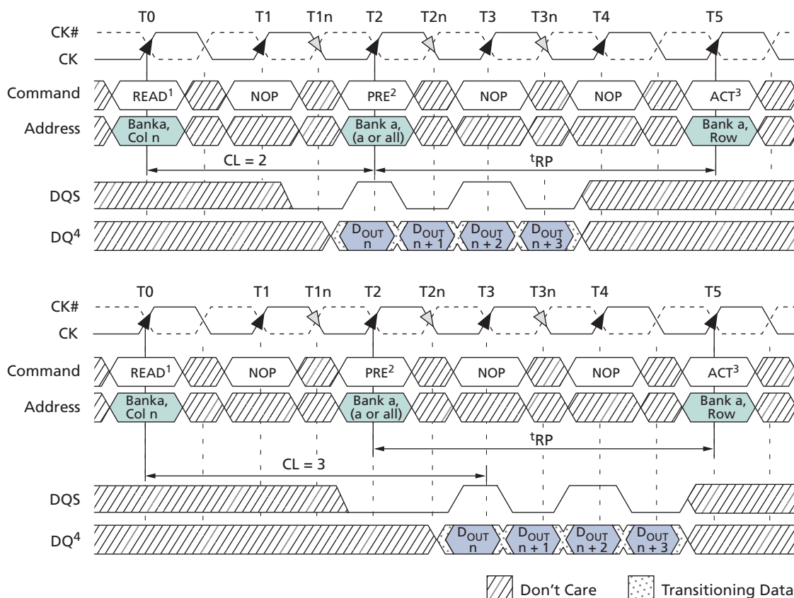
Figure 124: READ-to-PRECHARGE
