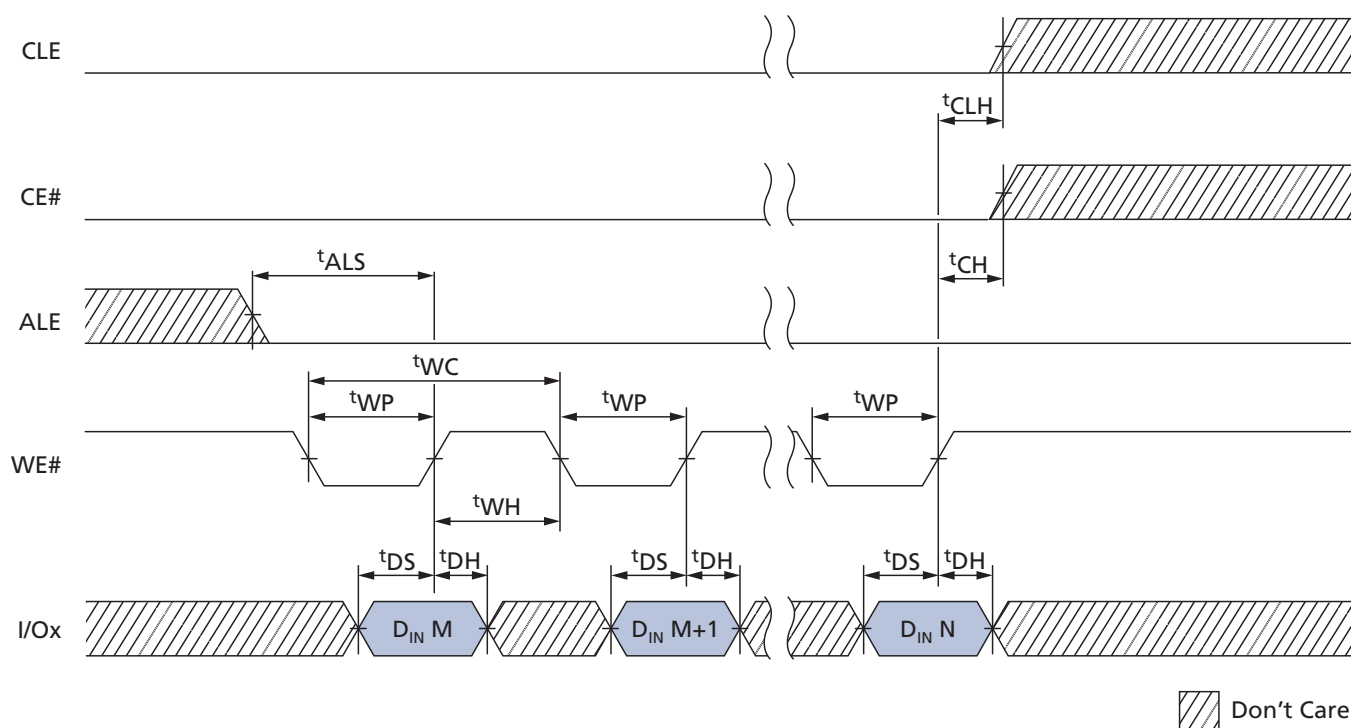
Figure 16: Asynchronous Data Input Cycles
