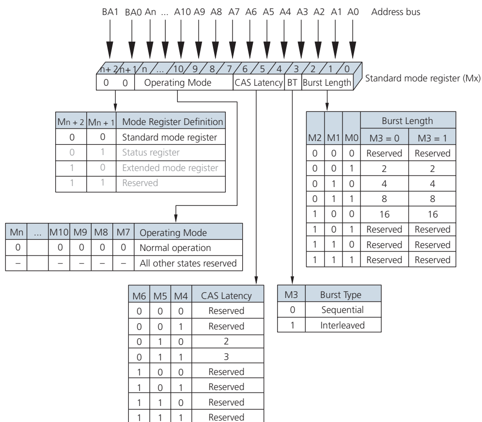
Figure 113: Standard Mode Register Definition
