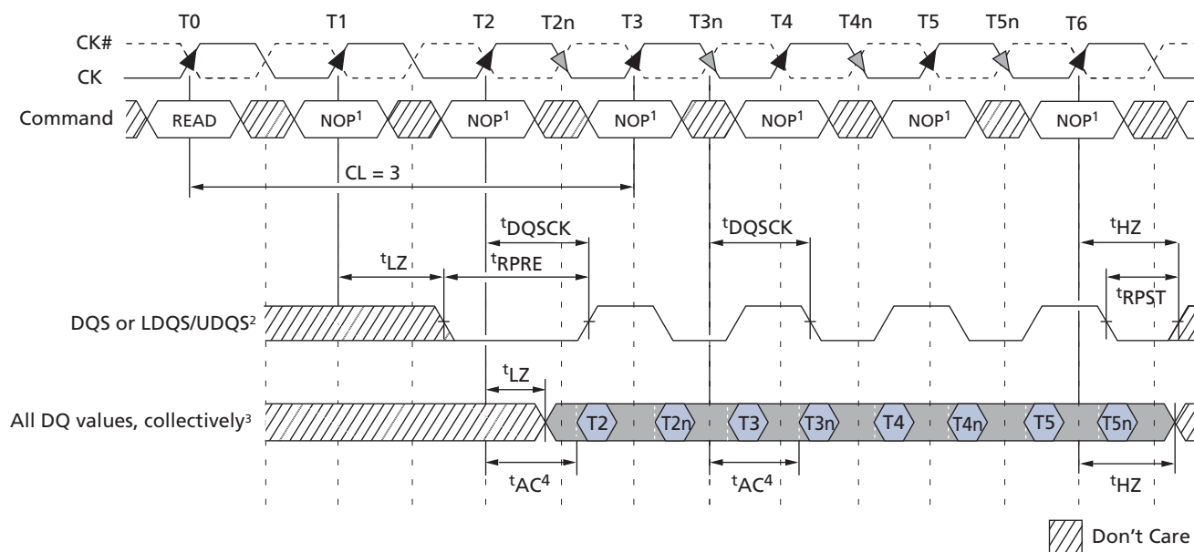
Figure 127: Data Output Timing – t_{AC} and t_{DQSCK}
