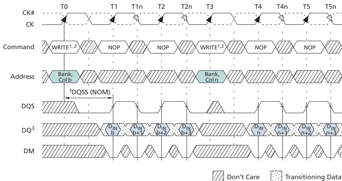
Figure 132: Nonconsecutive WRITE-to-WRITE
