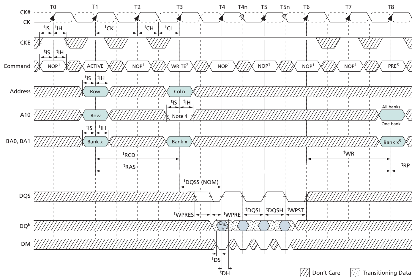
Figure 143: Bank Write – Without Auto Precharge
