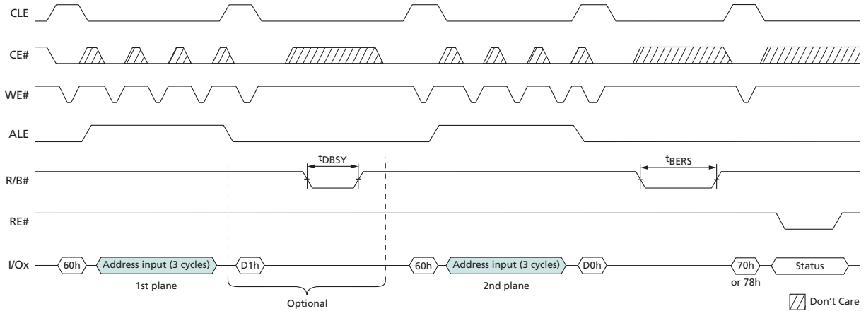
Figure 80: TWO-PLANE/MULTIPLE-DIE READ STATUS Cycle
