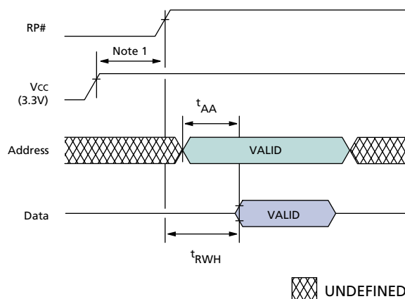
Figure 4: Power-Up/Reset Timing Diagram
