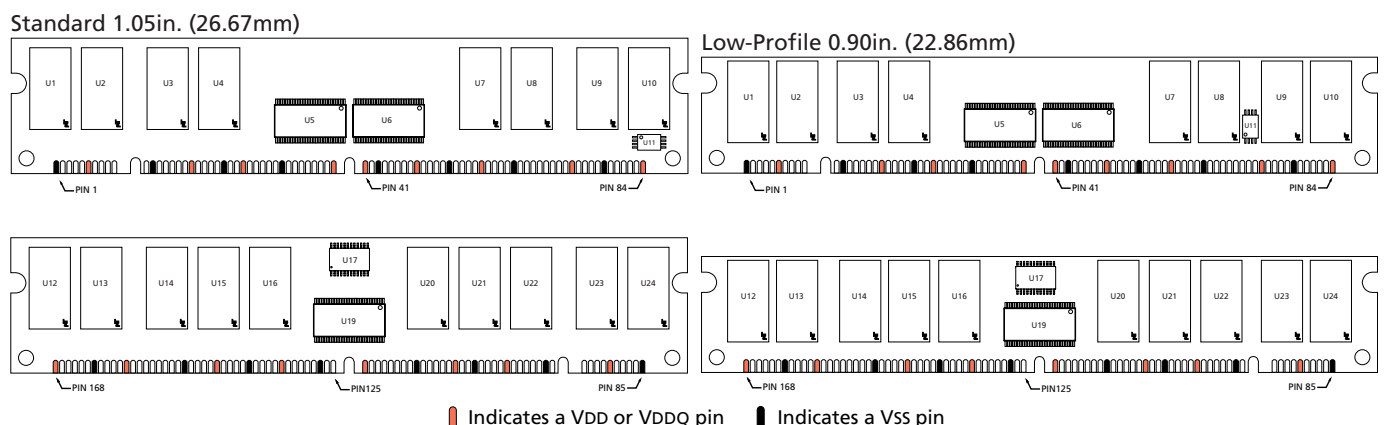
Figure 2: 168-Pin DIMM Pin Locations
