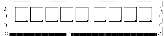
Figure 1: 240-Pin UDIMM (MO-269 R/C E)
