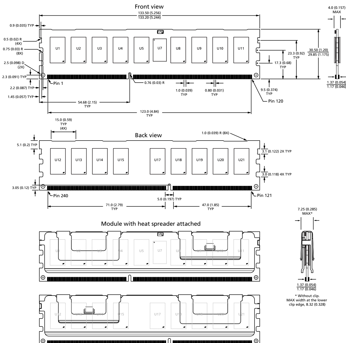
Figure 3: 240-Pin DDR3 RDIMM
