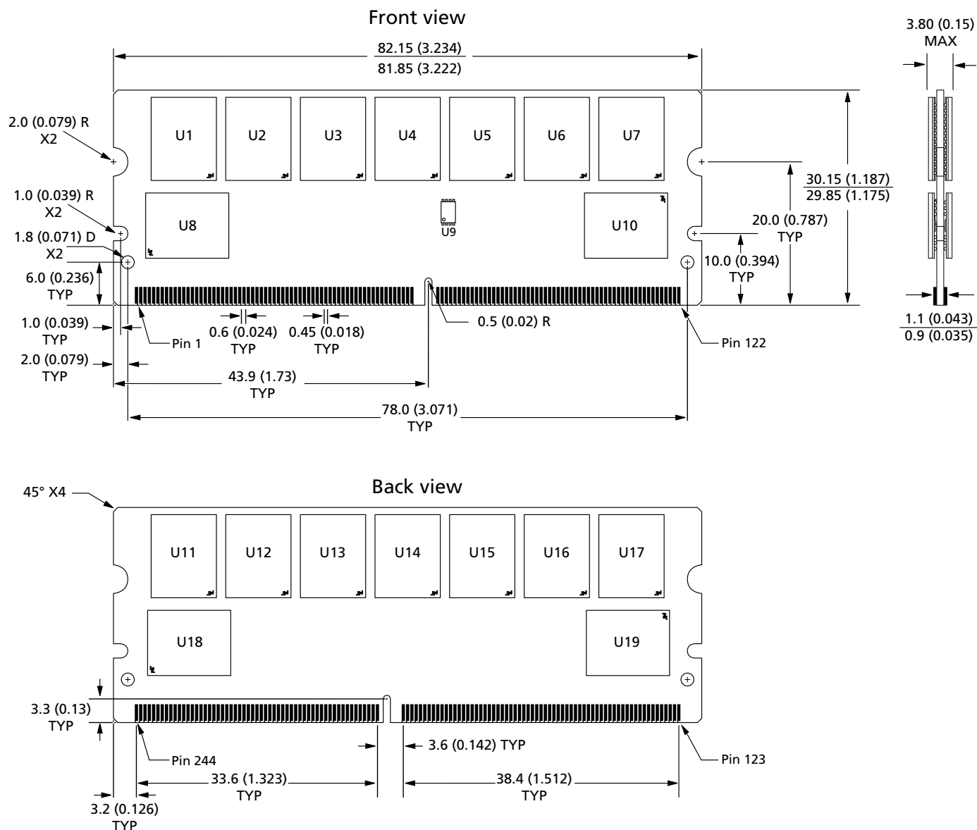
Figure 3: 244-Pin DDR3 Mini-UDIMM
