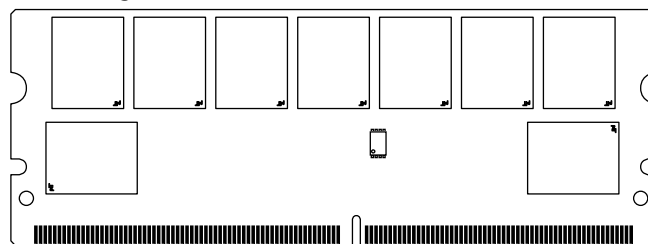
Figure 1: 244-Pin Mini-UDIMM (MO-244 R/C B)
