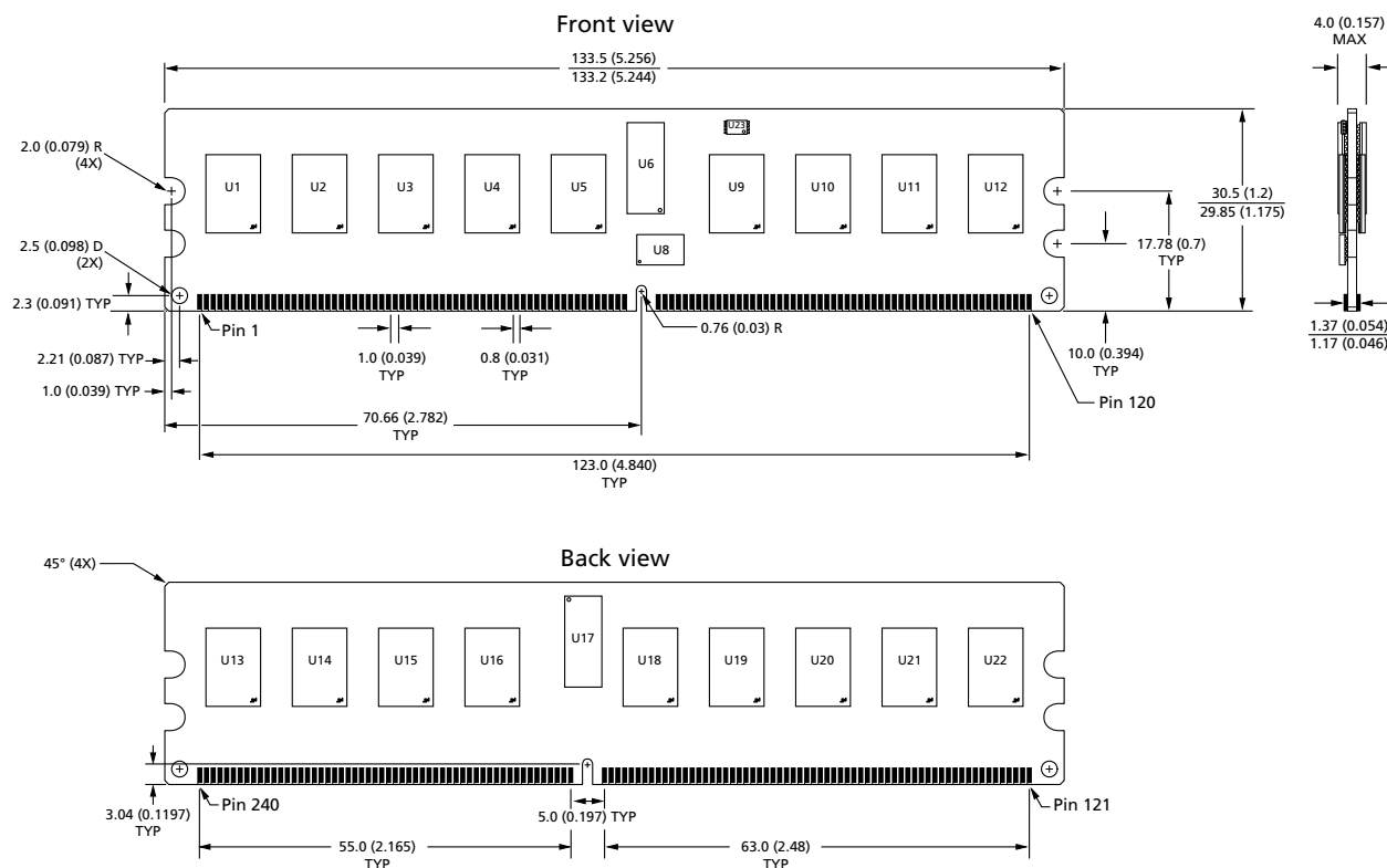
Figure 3: 240-Pin DDR2 RDIMM
