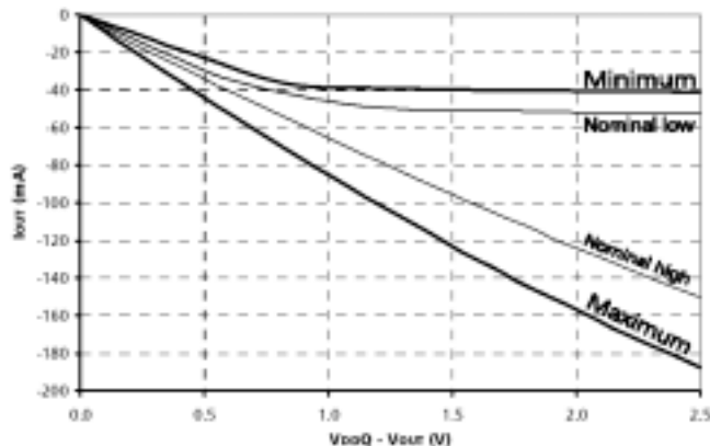
Figure 9: Pull-Up Characteristics
