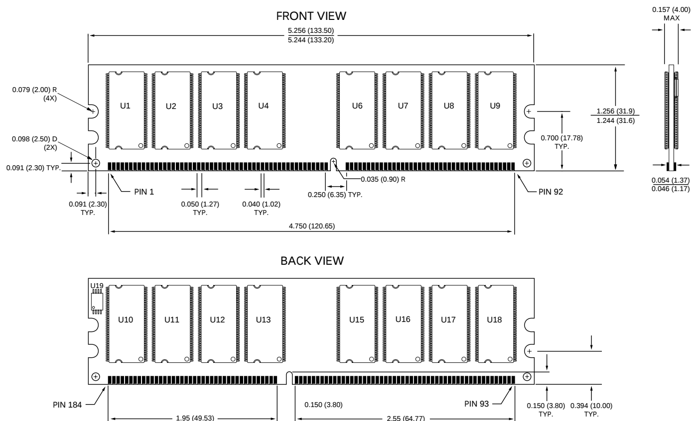
Figure 17: 184-PIN DDR DIMM Dimensions – Standard PCB
