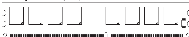
Figure 1: 184-Pin UDIMM (MO-206)
