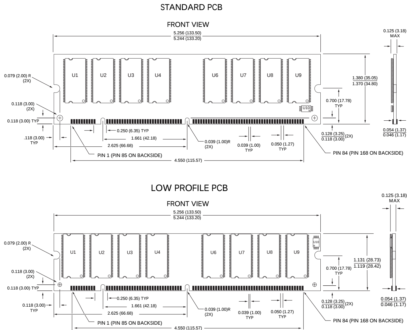
Figure 11: 168-Pin DIMM Dimensions – 512MB
