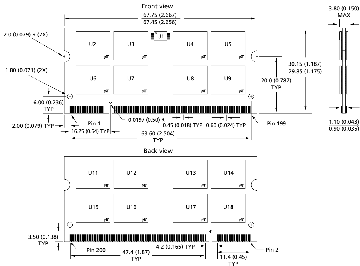
Figure 3: 200-Pin DDR2 SODIMM
