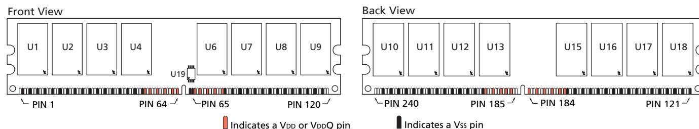
Figure 2: Pin Locations
