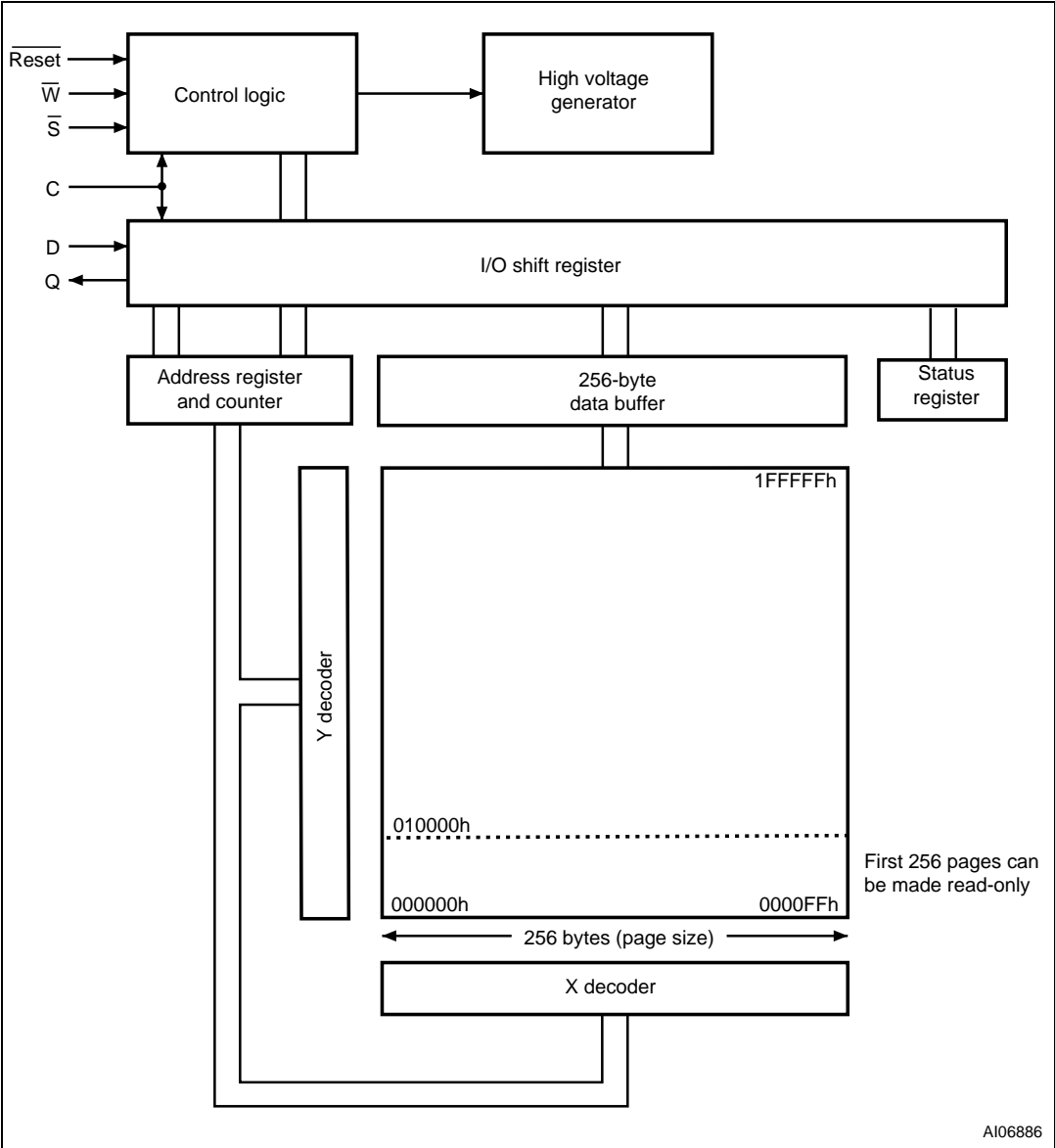
Figure 5. Block diagram
