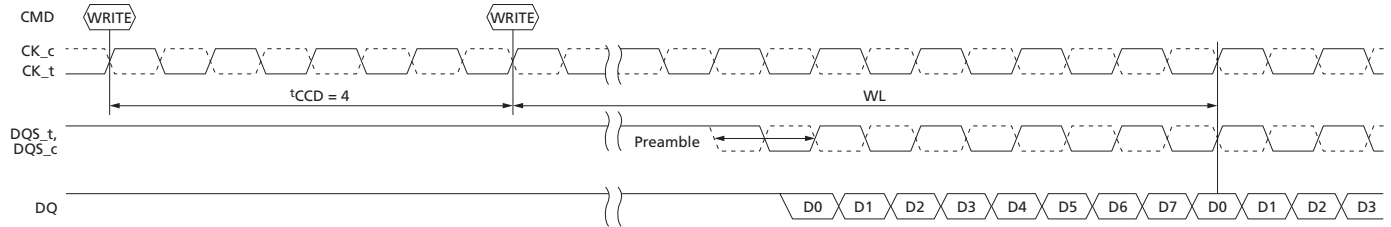
Figure 100: 1 t CK vs. 2 t CK WRITE Preamble Mode, t_{CCD} = 4
