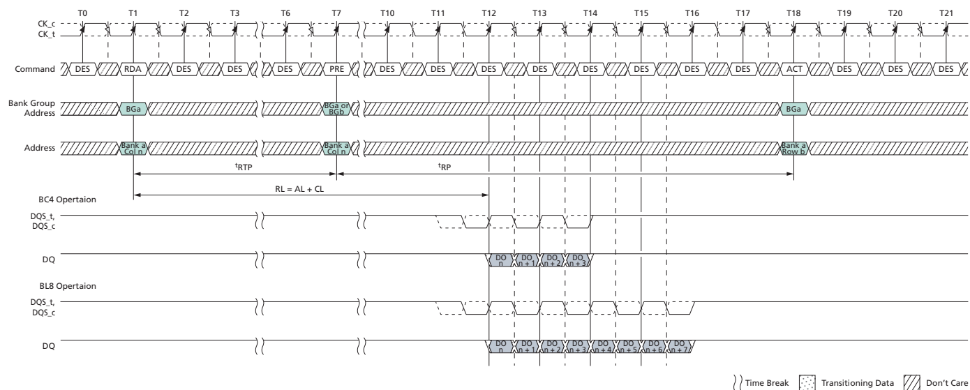
Figure 144: READ with Auto Precharge and 1t_{CK} Preamble
