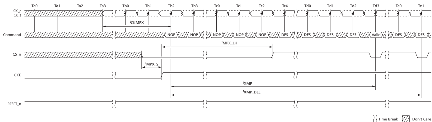
Figure 40: Maximum Power-Saving Mode Exit
