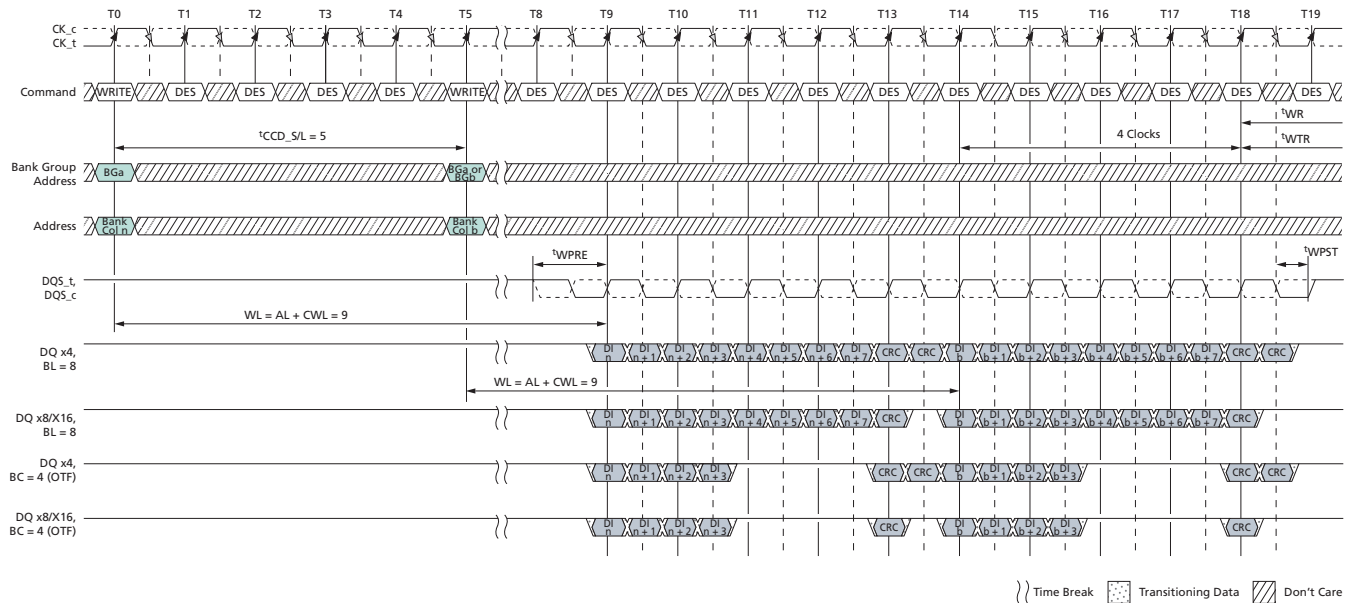
Figure 183: Consecutive WRITE (BL8/BC4-OTF) with 1 st CK Preamble and Write CRC in Same or Different Bank Group
