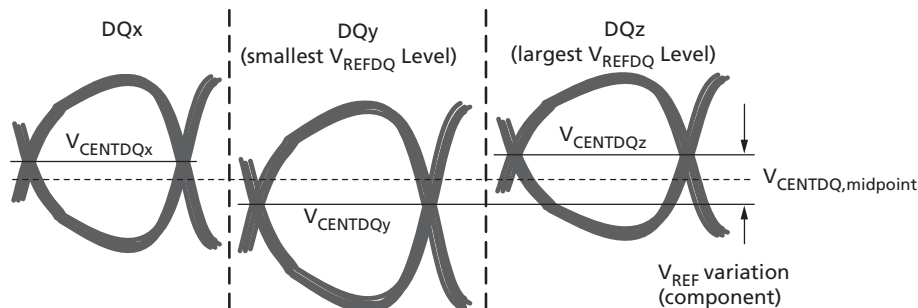
Figure 155: V_{\text{CENT\_DQ}} V_{\text{REFDQ}} Voltage Variation
