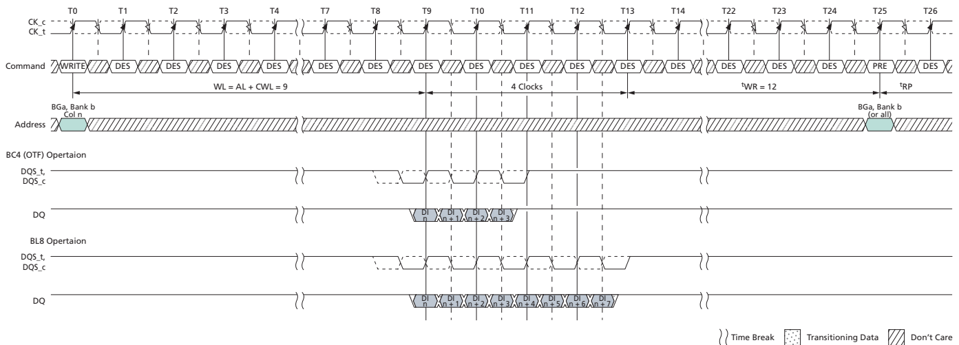
Figure 176: WRITE (BL8/BC4-OTF) to PRECHARGE with 1t_{CK} Preamble
