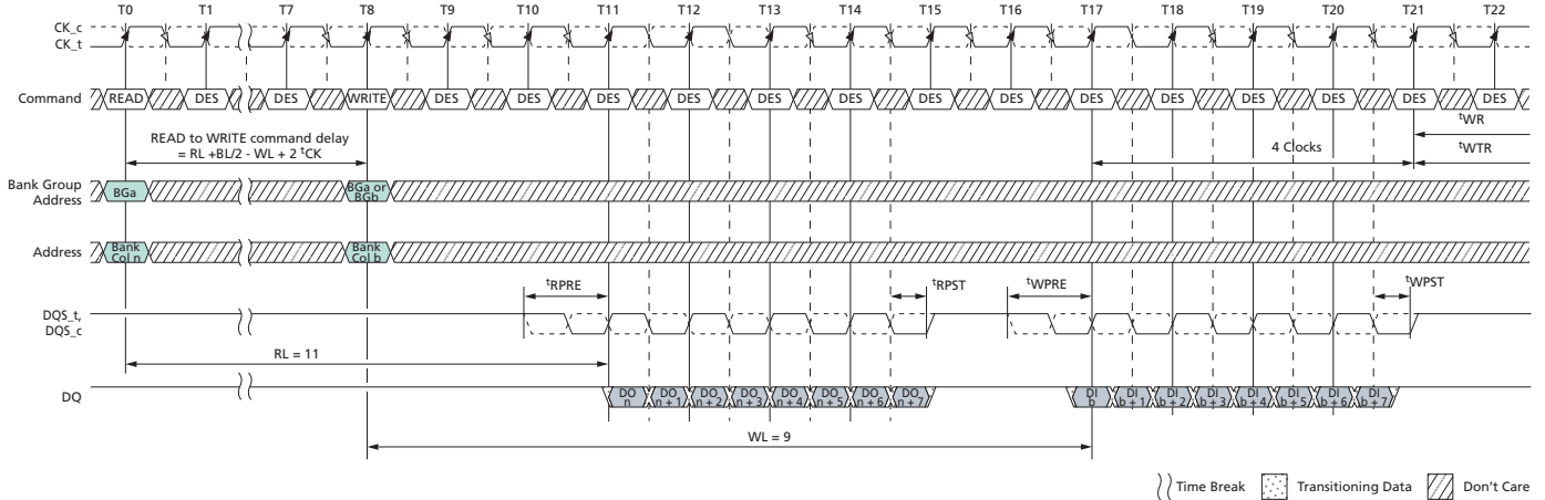
Figure 131: READ (BL8) to WRITE (BL8) with 1 t CK Preamble in Same or Different Bank Group
