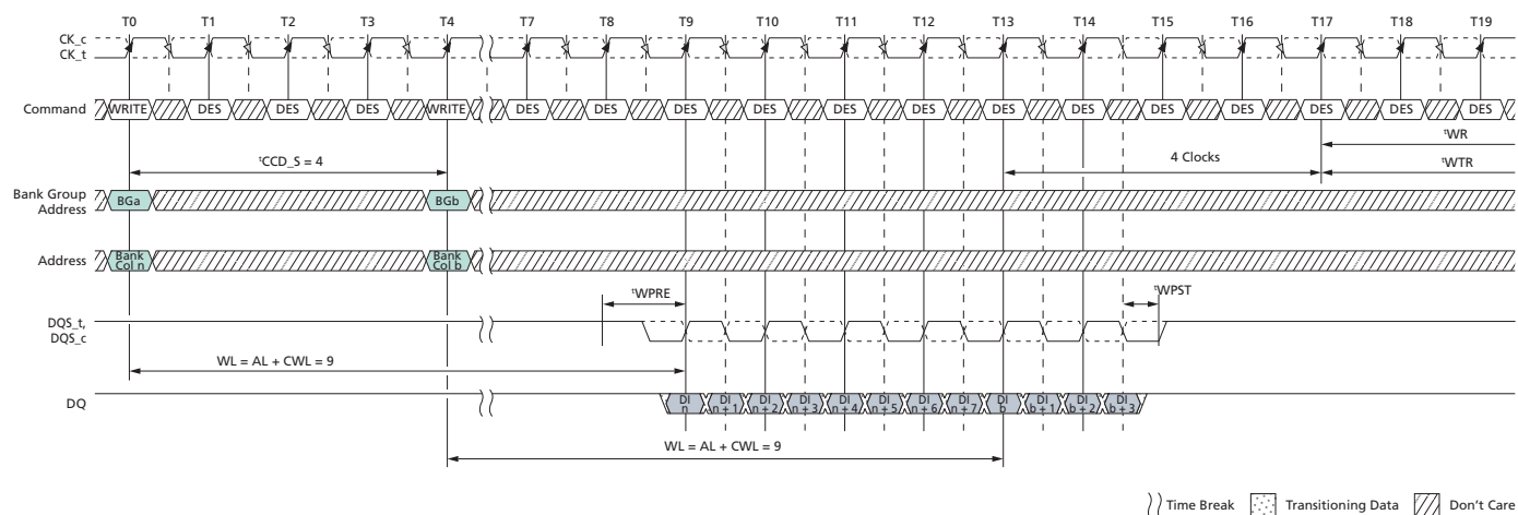
Figure 168: WRITE (BL8) to WRITE (BC4) OTF with 1^{\text{st}} CK Preamble in Different Bank Group
