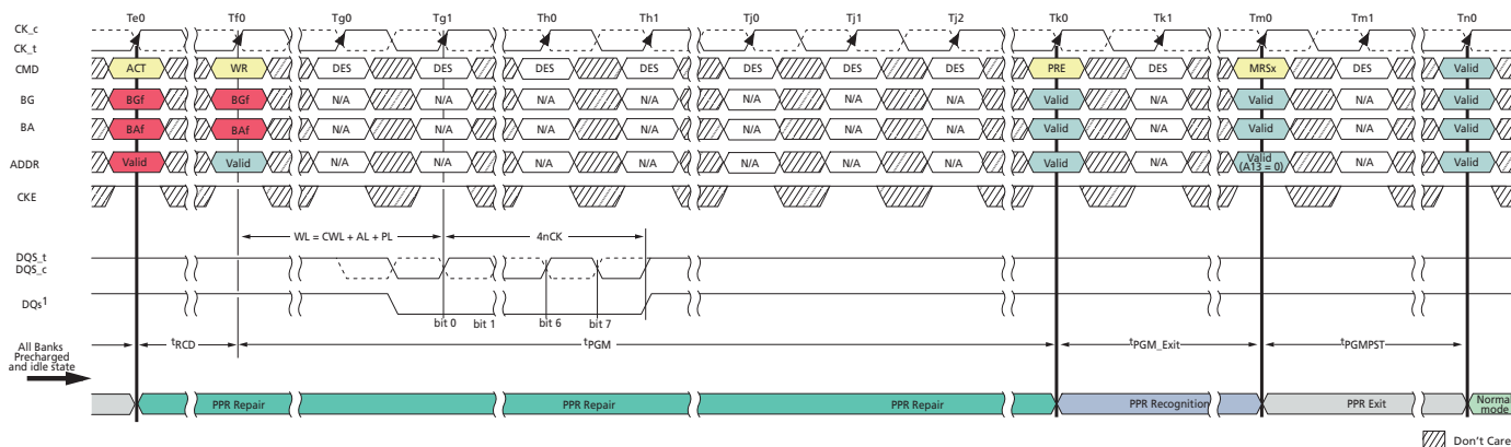
Figure 68: PPR WR – Repair and Exit
