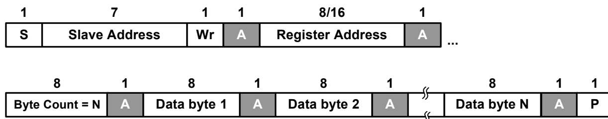
Figure 5.12 Block Write
