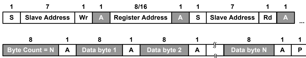
Figure 5.13 Block Read
