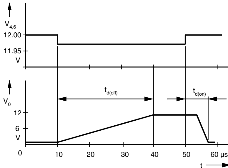
Figure 5-1. Delay Times
