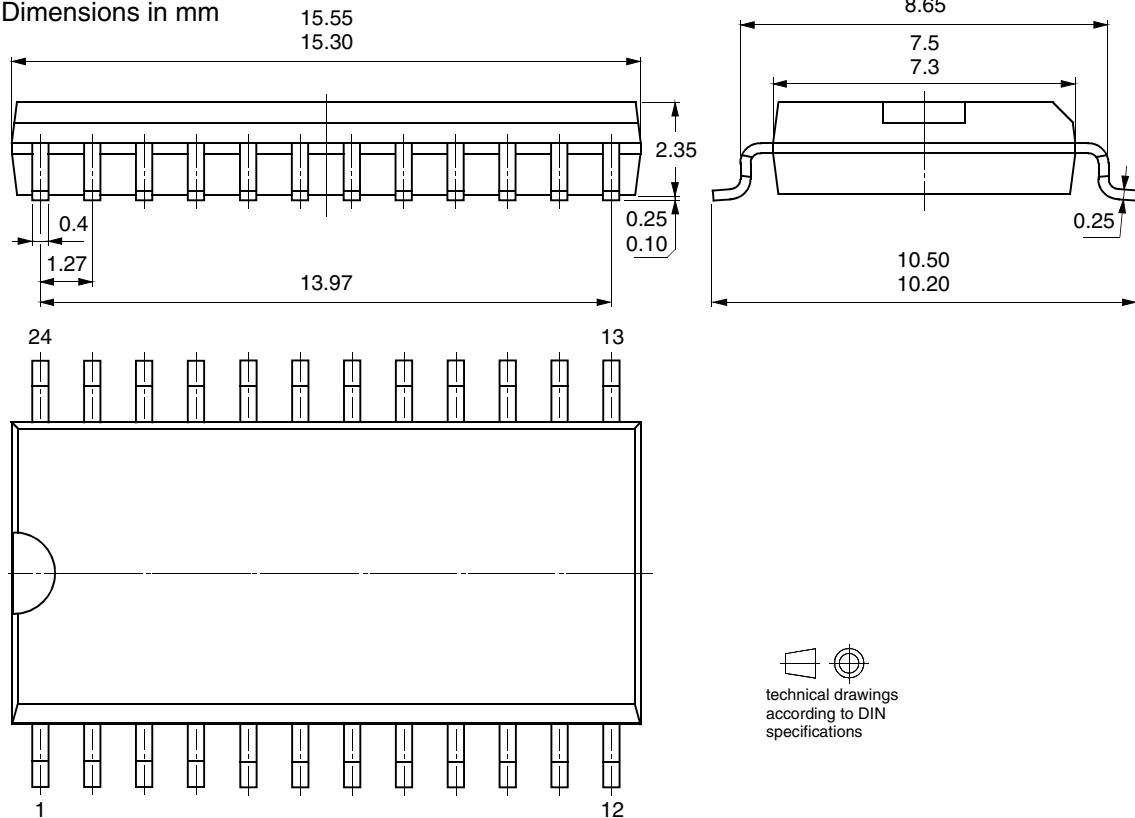
Package SO24 Dimensions in mm
