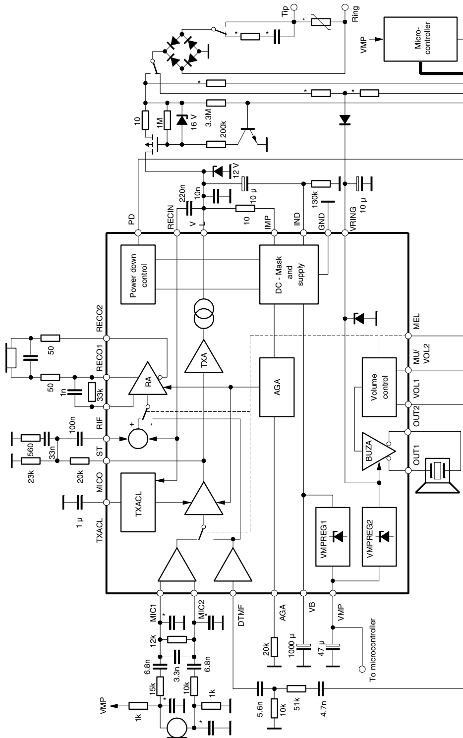
Figure 2-2. Detailed Block Diagram with External Components
