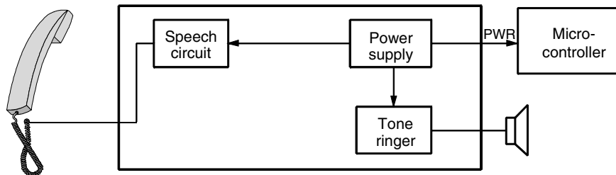
Figure 1-1. Block Diagram
