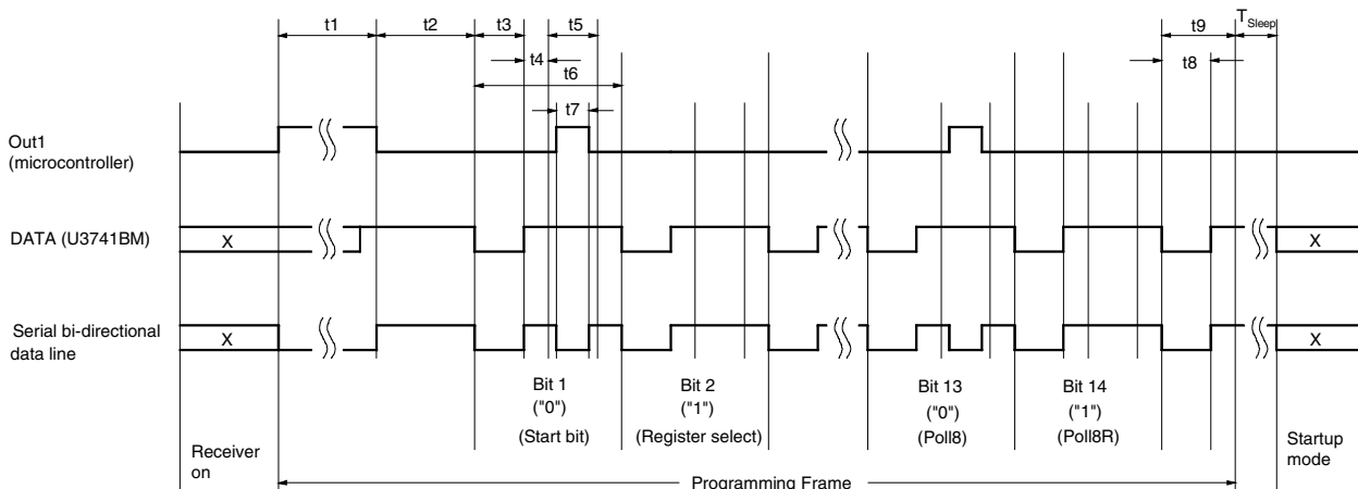
Figure 20. Timing of the Register Programming
